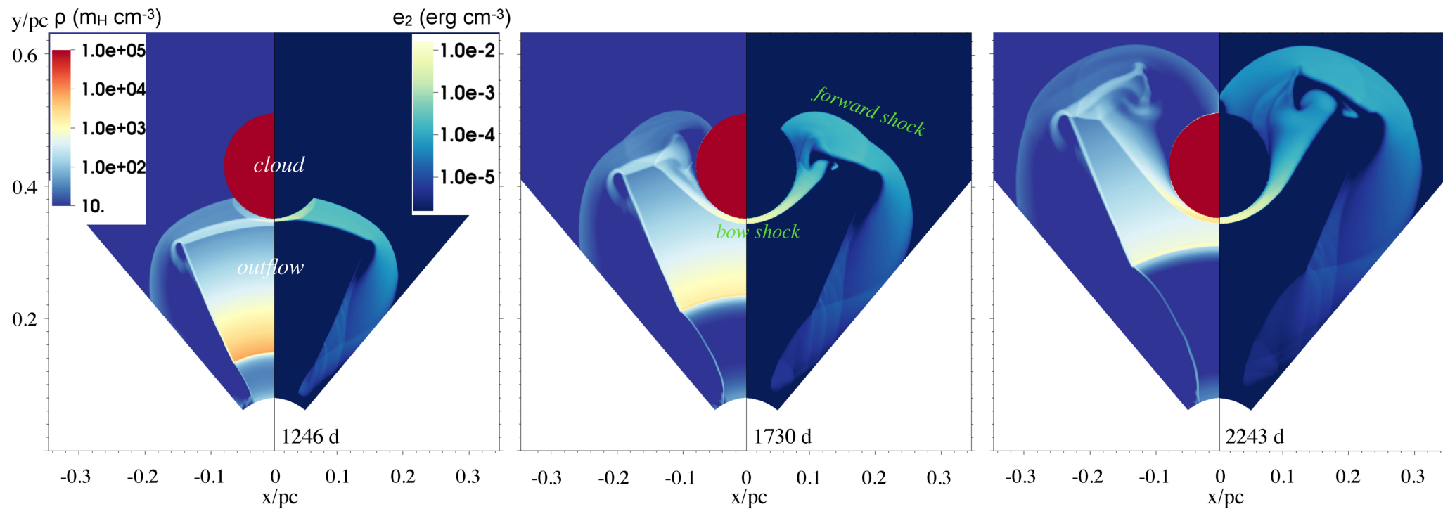
Figure 5. from Lei Yang et al 2025 Astrophys. J. Lett. 993 doi:10.3847/2041-8213/ae0caa https://dx.doi.org/10.3847/2041-8213/ae0caa © 2025. The Author(s). Published by the American Astronomical Society.
