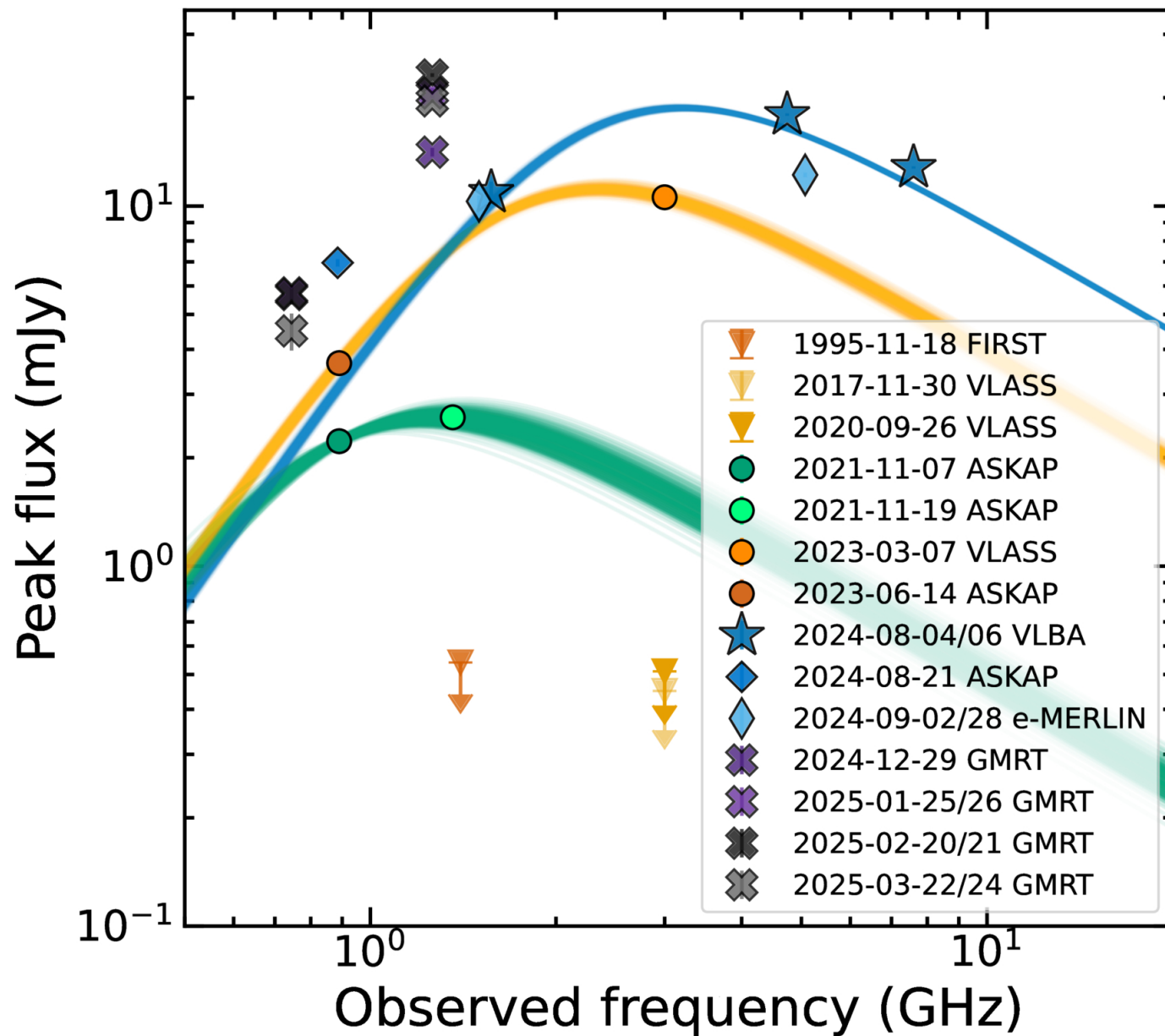
Figure 3. from Lei Yang et al 2025 Astrophys. J. Lett. 993 doi:10.3847/2041-8213/ae0caa https://dx.doi.org/10.3847/2041-8213/ae0caa © 2025. The Author(s). Published by the American Astronomical Society.
