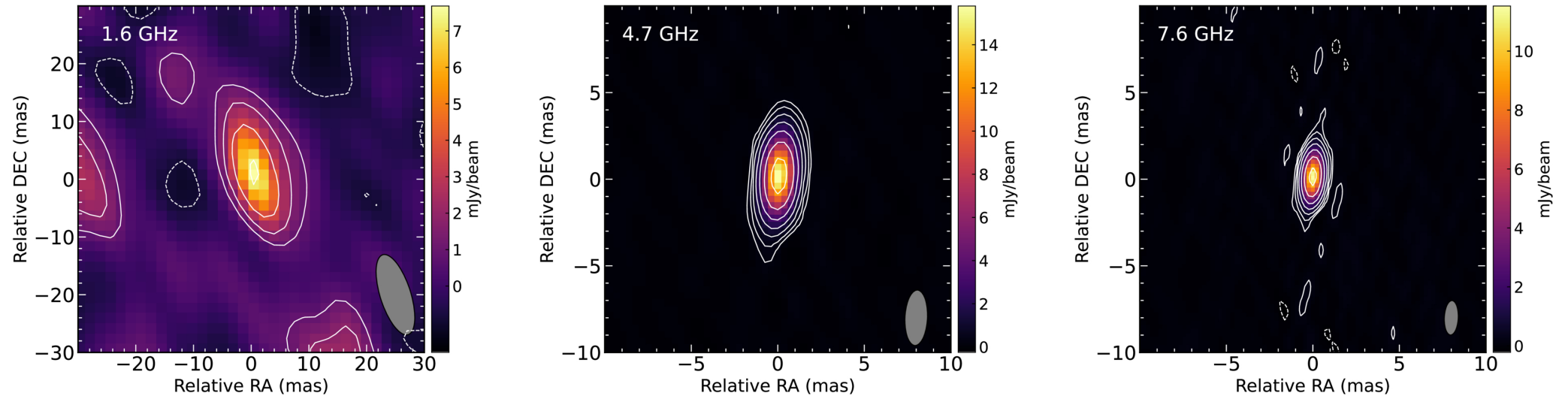
Figure 1. from Lei Yang et al 2025 Astrophys. J. Lett. 993 doi:10.3847/2041-8213/ae0caa https://dx.doi.org/10.3847/2041-8213/ae0caa © 2025. The Author(s). Published by the American Astronomical Society.
