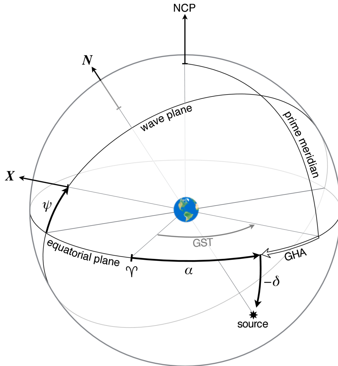
Figure 4. from A. G. Abac et al 2025 Astrophys. J. Lett. 995 doi:10.3847/2041-8213/ae0c06 https://dx.doi.org/10.3847/2041-8213/ae0c06 © 2025. The Author(s). Published by the American Astronomical Society.
