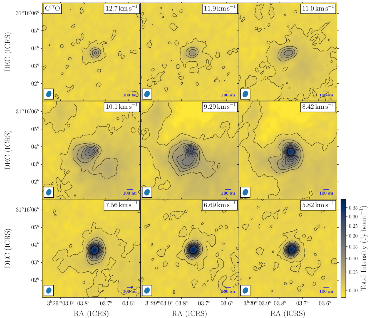
Figure 4. from P. C. Cortés et al 2025 Astrophys. J. Lett. 992 doi:10.3847/2041-8213/ae0c04 https://dx.doi.org/10.3847/2041-8213/ae0c04 © 2025. The Author(s). Published by the American Astronomical Society.
