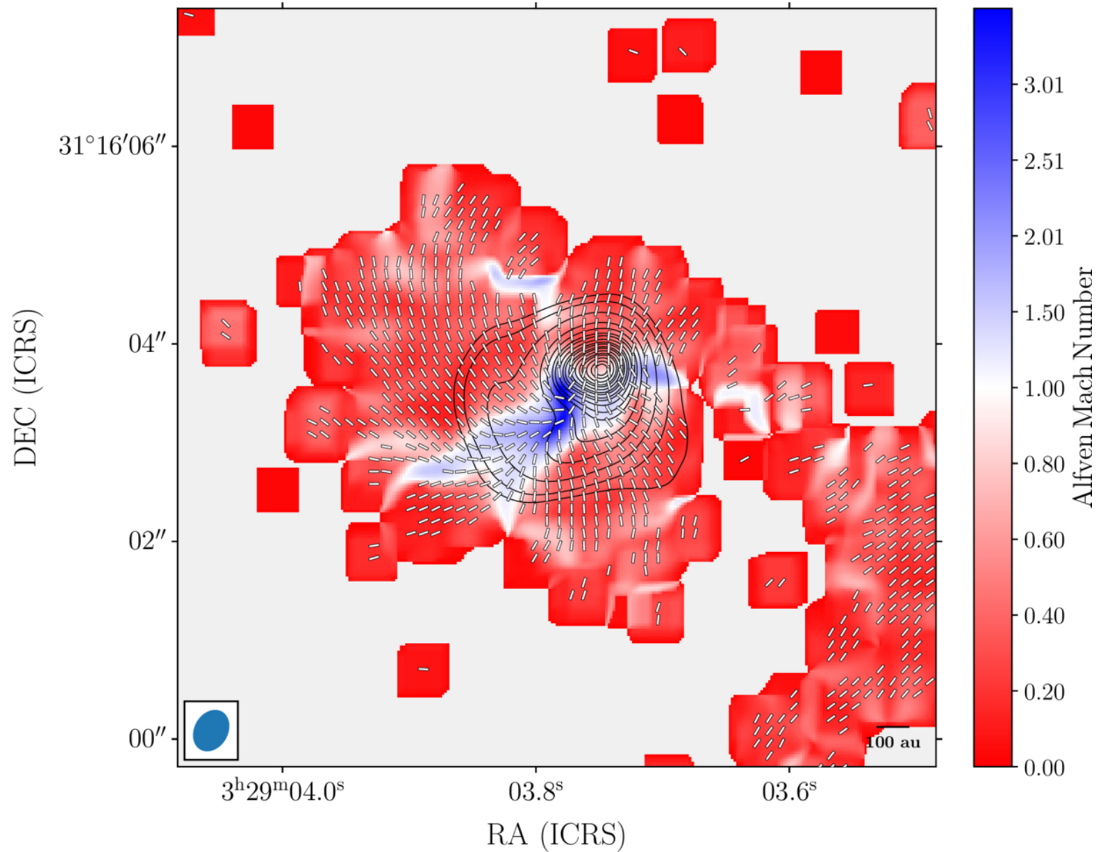
Figure 17. from P. C. Cortés et al 2025 Astrophys. J. Lett. 992 doi:10.3847/2041-8213/ae0c04 https://dx.doi.org/10.3847/2041-8213/ae0c04 © 2025. The Author(s). Published by the American Astronomical Society.
