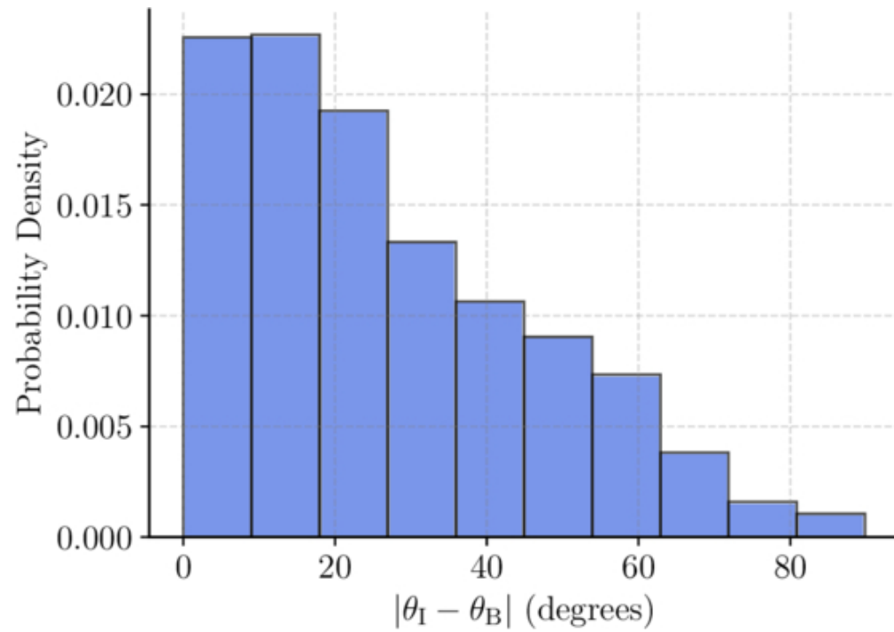
Figure 15. from P. C. Cortés et al 2025 Astrophys. J. Lett. 992 doi:10.3847/2041-8213/ae0c04 https://dx.doi.org/10.3847/2041-8213/ae0c04 © 2025. The Author(s). Published by the American Astronomical Society.
