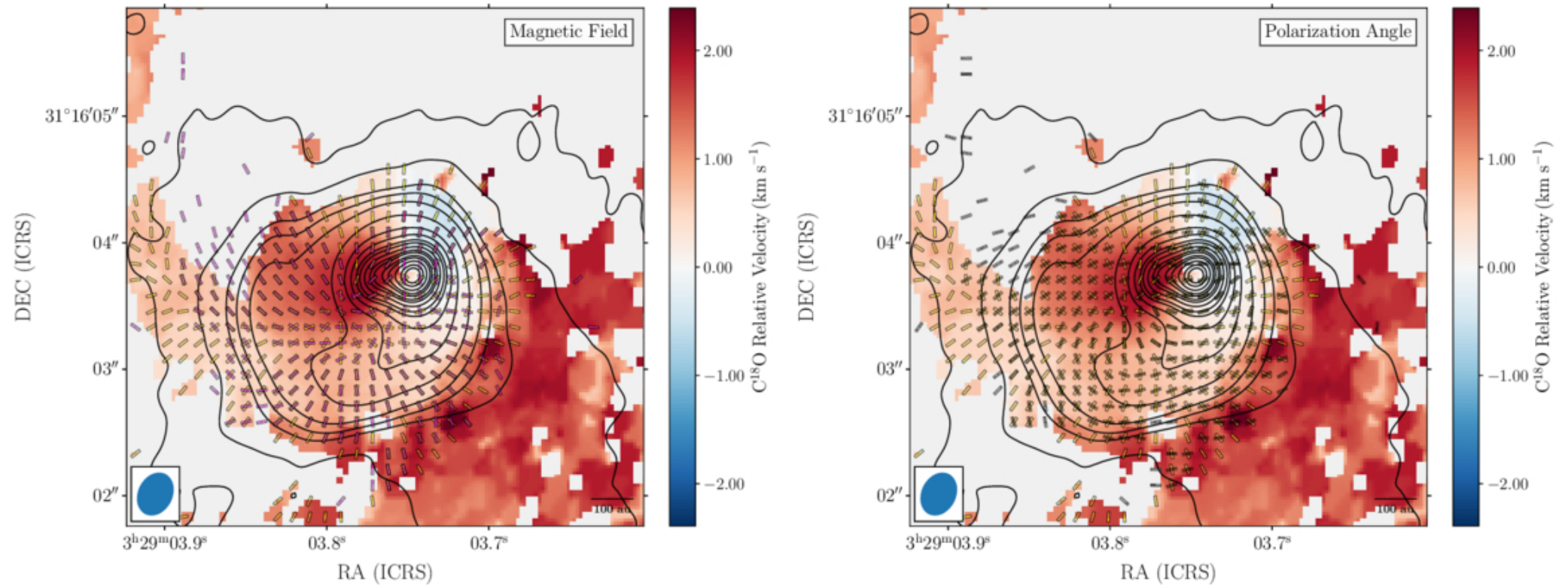
Figure 14. from P. C. Cortés et al 2025 Astrophys. J. Lett. 992 doi:10.3847/2041-8213/ae0c04 https://dx.doi.org/10.3847/2041-8213/ae0c04 © 2025. The Author(s). Published by the American Astronomical Society.
