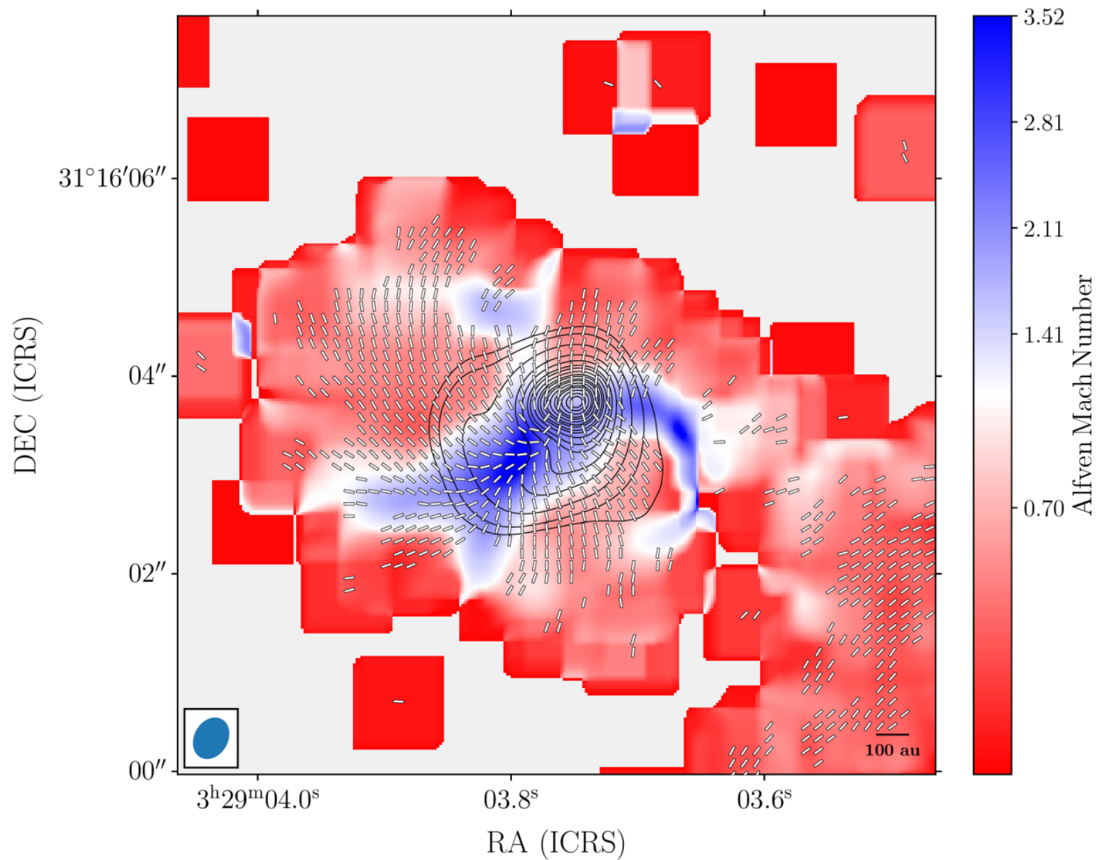
Figure 12. from P. C. Cortés et al 2025 Astrophys. J. Lett. 992 doi:10.3847/2041-8213/ae0c04 https://dx.doi.org/10.3847/2041-8213/ae0c04 © 2025. The Author(s). Published by the American Astronomical Society.
