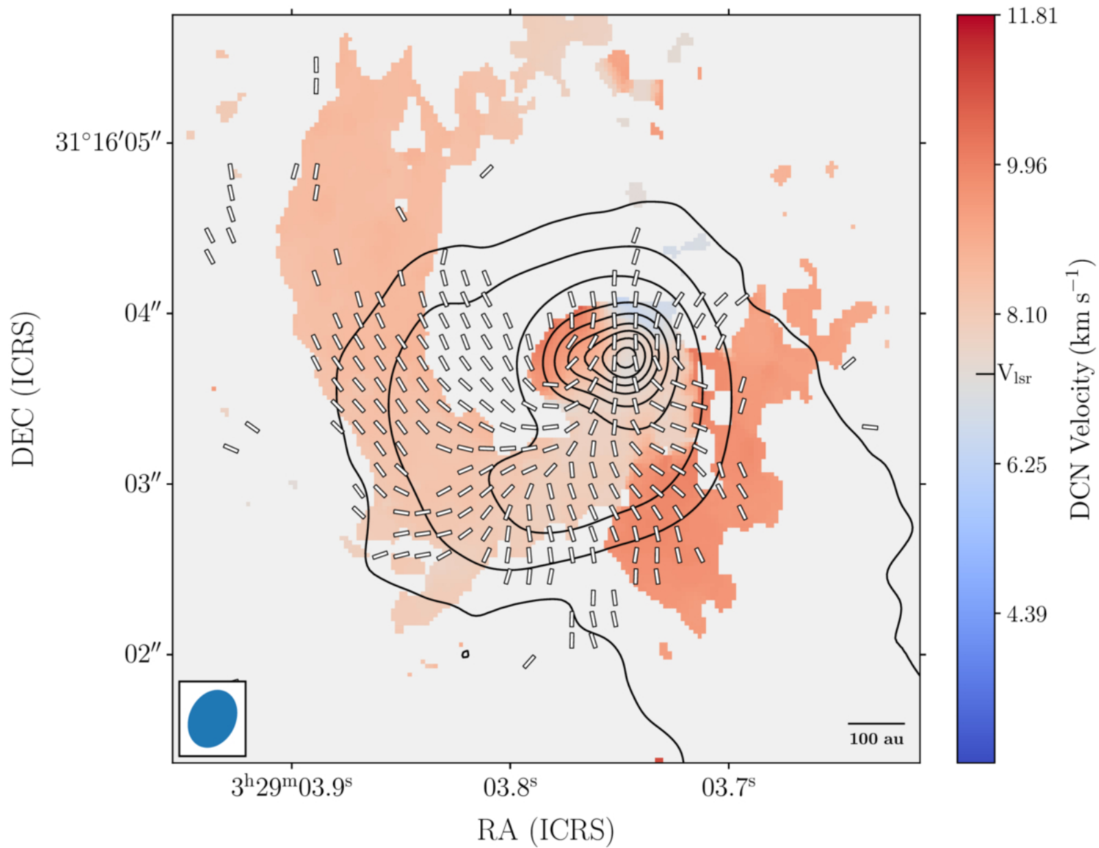
Figure 11. from P. C. Cortés et al 2025 Astrophys. J. Lett. 992 doi:10.3847/2041-8213/ae0c04 https://dx.doi.org/10.3847/2041-8213/ae0c04 © 2025. The Author(s). Published by the American Astronomical Society.
