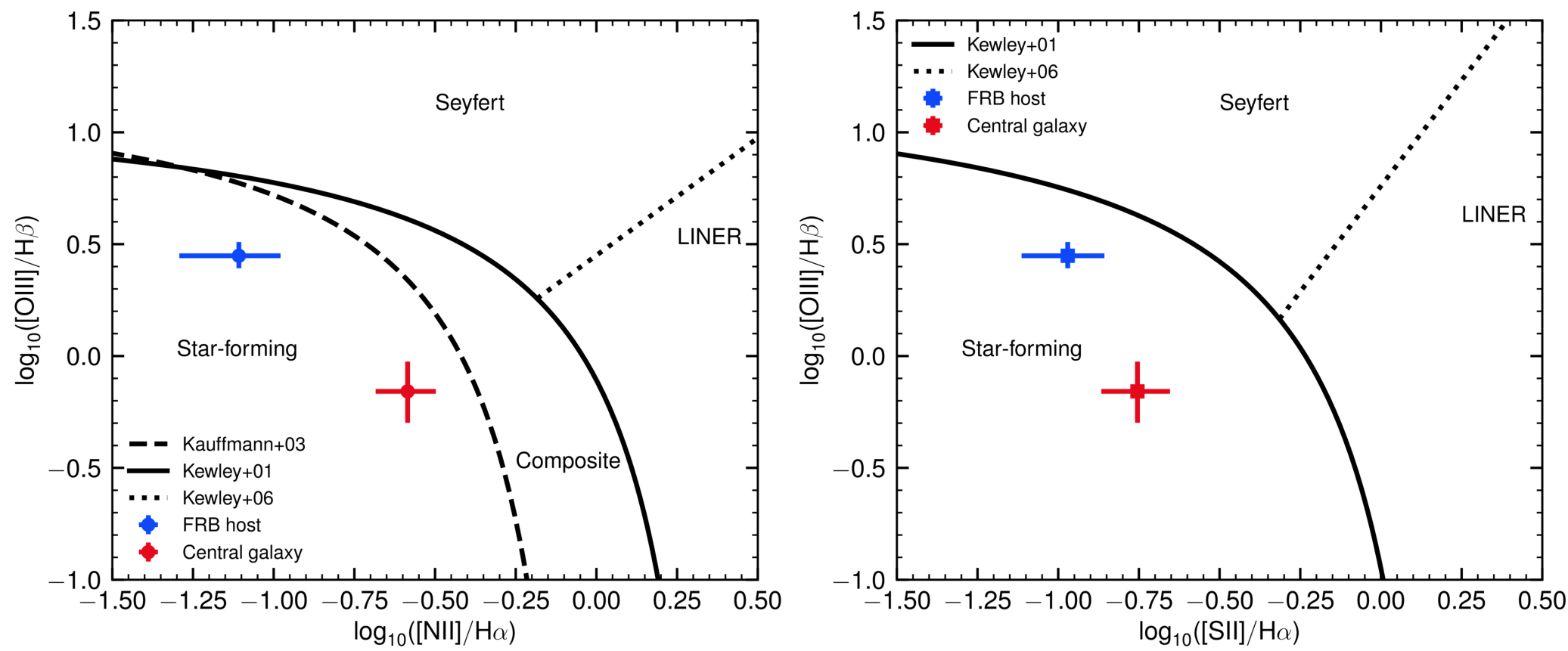
Figure 9. from M. Bhardwaj et al 2025 Astrophys. J. Lett. 992 doi:10.3847/2041-8213/ae0b68 https://dx.doi.org/10.3847/2041-8213/ae0b68 © 2025. The Author(s). Published by the American Astronomical Society.
