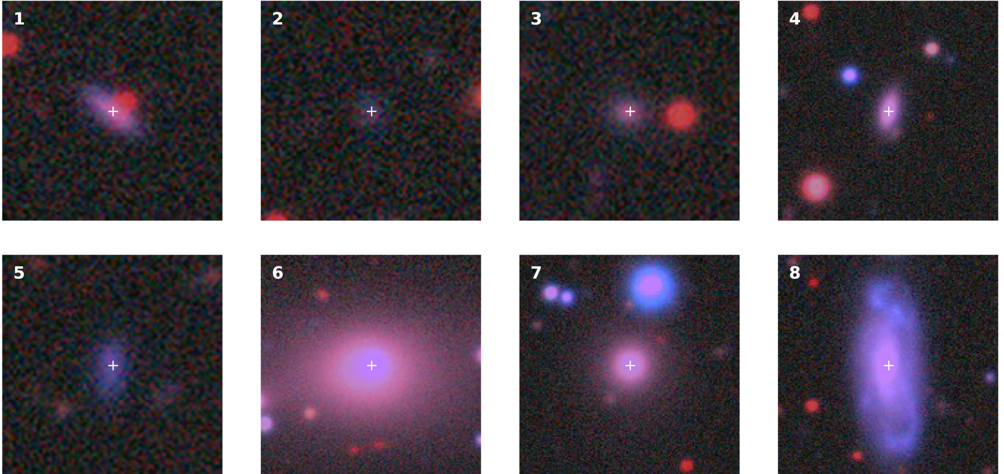
Figure 8. from M. Bhardwaj et al 2025 Astrophys. J. Lett. 992 doi:10.3847/2041-8213/ae0b68 https://dx.doi.org/10.3847/2041-8213/ae0b68 © 2025. The Author(s). Published by the American Astronomical Society.
