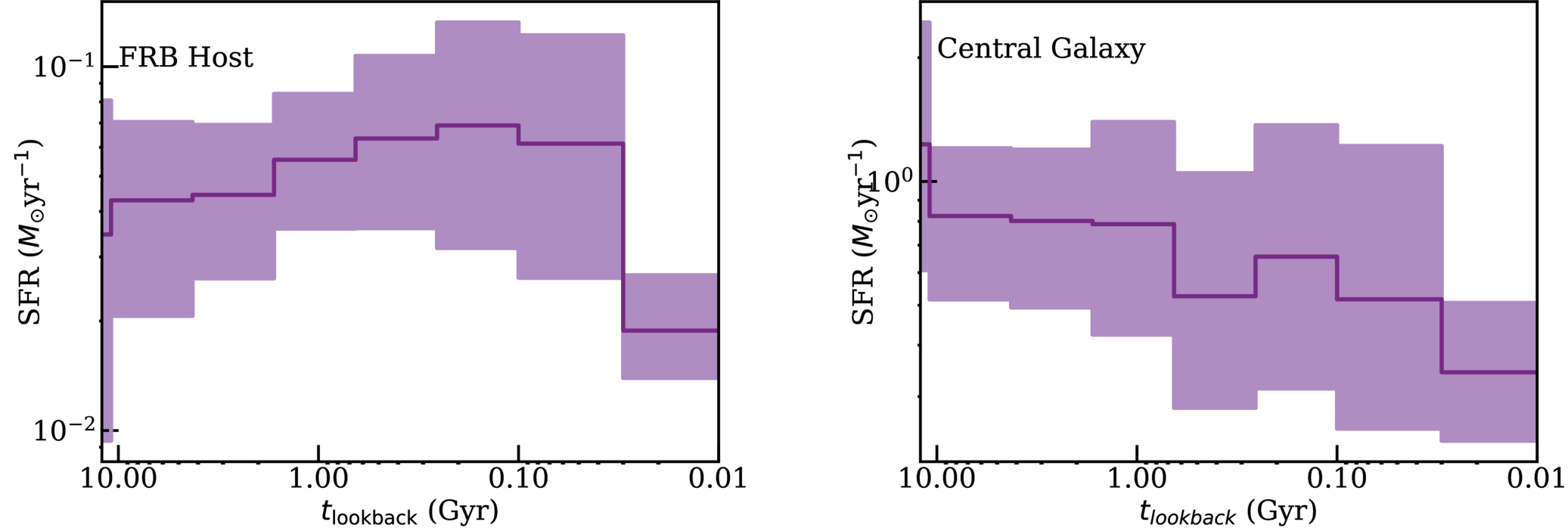
Figure 5. from M. Bhardwaj et al 2025 Astrophys. J. Lett. 992 doi:10.3847/2041-8213/ae0b68 https://dx.doi.org/10.3847/2041-8213/ae0b68 © 2025. The Author(s). Published by the American Astronomical Society.
