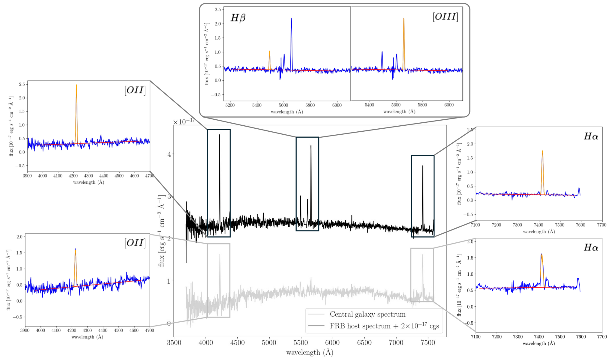
Figure 4. from M. Bhardwaj et al 2025 Astrophys. J. Lett. 992 doi:10.3847/2041-8213/ae0b68 https://dx.doi.org/10.3847/2041-8213/ae0b68 © 2025. The Author(s). Published by the American Astronomical Society.
