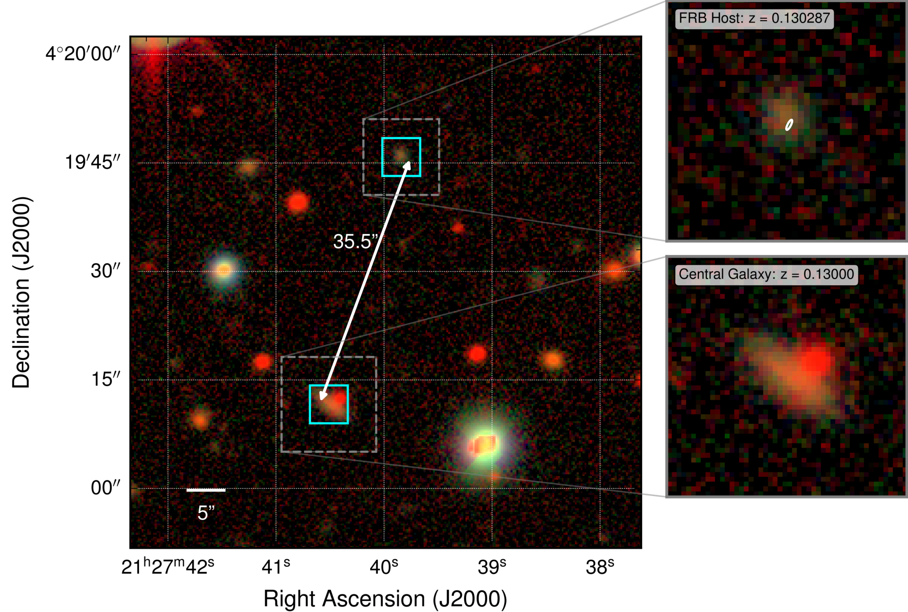
Figure 3. from M. Bhardwaj et al 2025 Astrophys. J. Lett. 992 doi:10.3847/2041-8213/ae0b68 https://dx.doi.org/10.3847/2041-8213/ae0b68 © 2025. The Author(s). Published by the American Astronomical Society.
