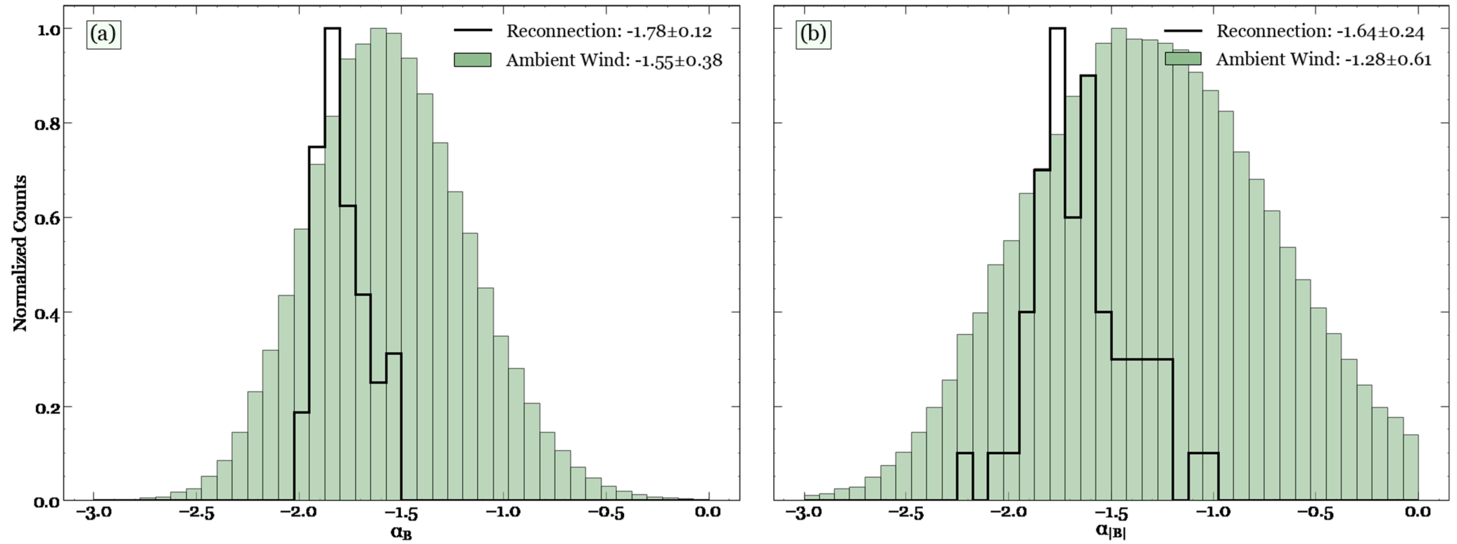
Figure 5. from Tamar Ervin et al 2025 Astrophys. J. Lett. 992 doi:10.3847/2041-8213/ae0b56 https://dx.doi.org/10.3847/2041-8213/ae0b56 © 2025. The Author(s). Published by the American Astronomical Society.
