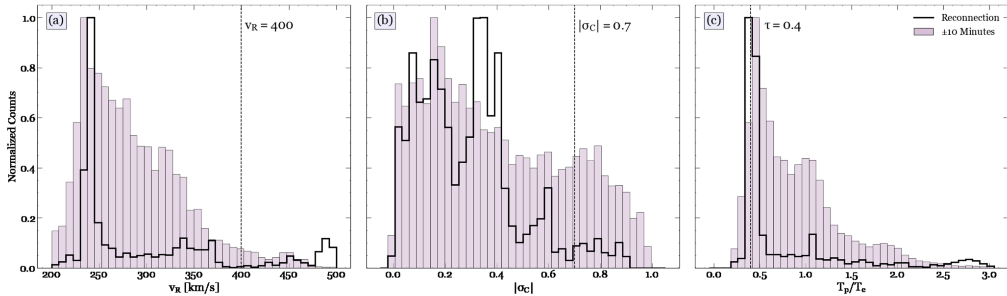
Figure 4. from Tamar Ervin et al 2025 Astrophys. J. Lett. 992 doi:10.3847/2041-8213/ae0b56 https://dx.doi.org/10.3847/2041-8213/ae0b56 © 2025. The Author(s). Published by the American Astronomical Society.
