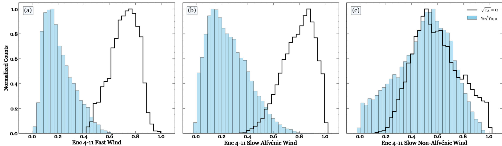
Figure 3. from Tamar Ervin et al 2025 Astrophys. J. Lett. 992 doi:10.3847/2041-8213/ae0b56 https://dx.doi.org/10.3847/2041-8213/ae0b56 © 2025. The Author(s). Published by the American Astronomical Society.
