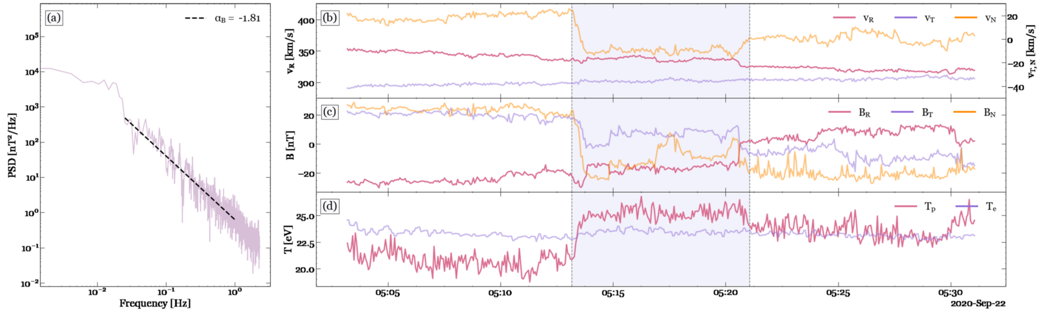
Figure 1. from Tamar Ervin et al 2025 Astrophys. J. Lett. 992 doi:10.3847/2041-8213/ae0b56 https://dx.doi.org/10.3847/2041-8213/ae0b56 © 2025. The Author(s). Published by the American Astronomical Society.
