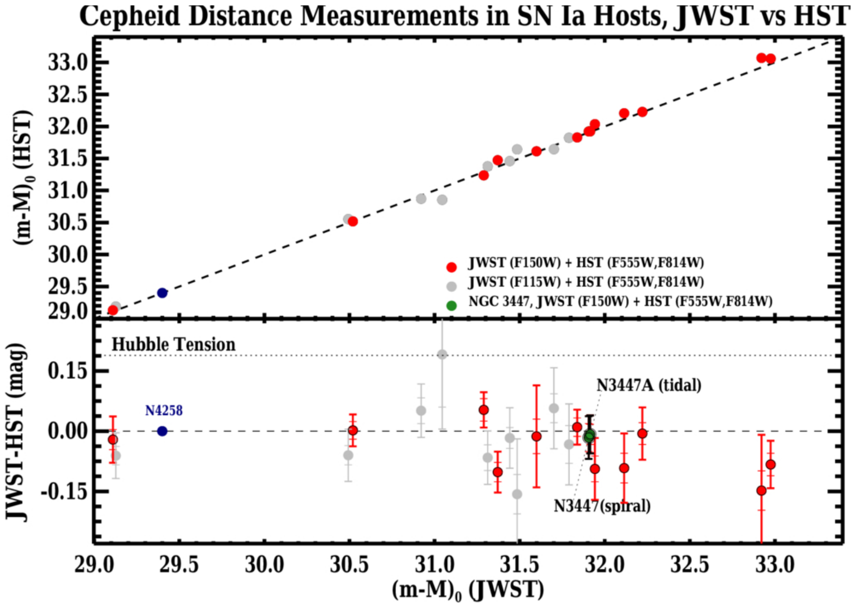
Figure 9. from Adam G. Riess et al 2025 Astrophys. J. Lett. 992 doi:10.3847/2041-8213/ae0ad6 https://dx.doi.org/10.3847/2041-8213/ae0ad6 © 2025. The Author(s). Published by the American Astronomical Society.
