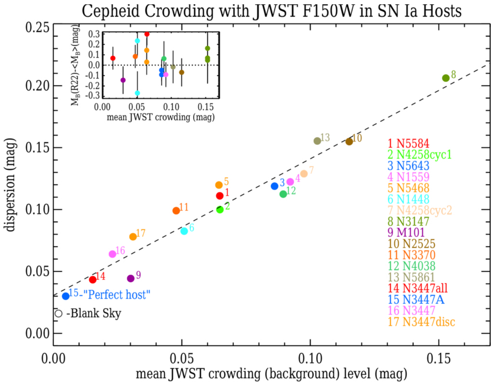
Figure 7. from Adam G. Riess et al 2025 Astrophys. J. Lett. 992 doi:10.3847/2041-8213/ae0ad6 https://dx.doi.org/10.3847/2041-8213/ae0ad6 © 2025. The Author(s). Published by the American Astronomical Society.
