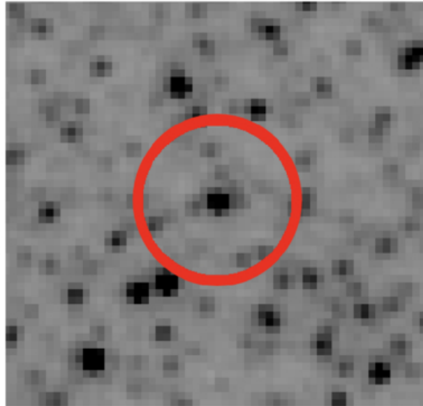
JWST NIRCAM F150W
