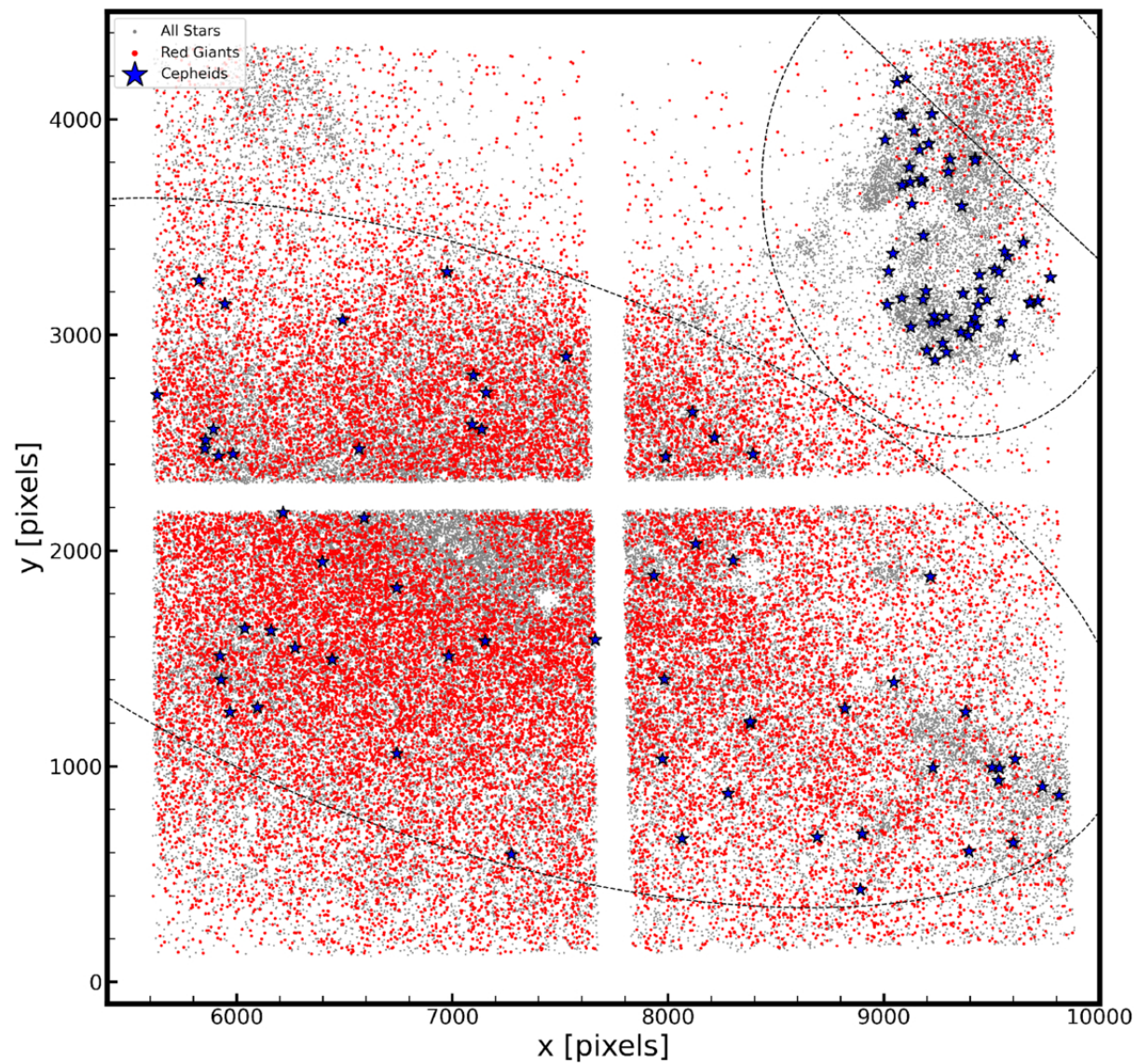
Figure 4. from Adam G. Riess et al 2025 Astrophys. J. Lett. 992 doi:10.3847/2041-8213/ae0ad6 https://dx.doi.org/10.3847/2041-8213/ae0ad6 © 2025. The Author(s). Published by the American Astronomical Society.
