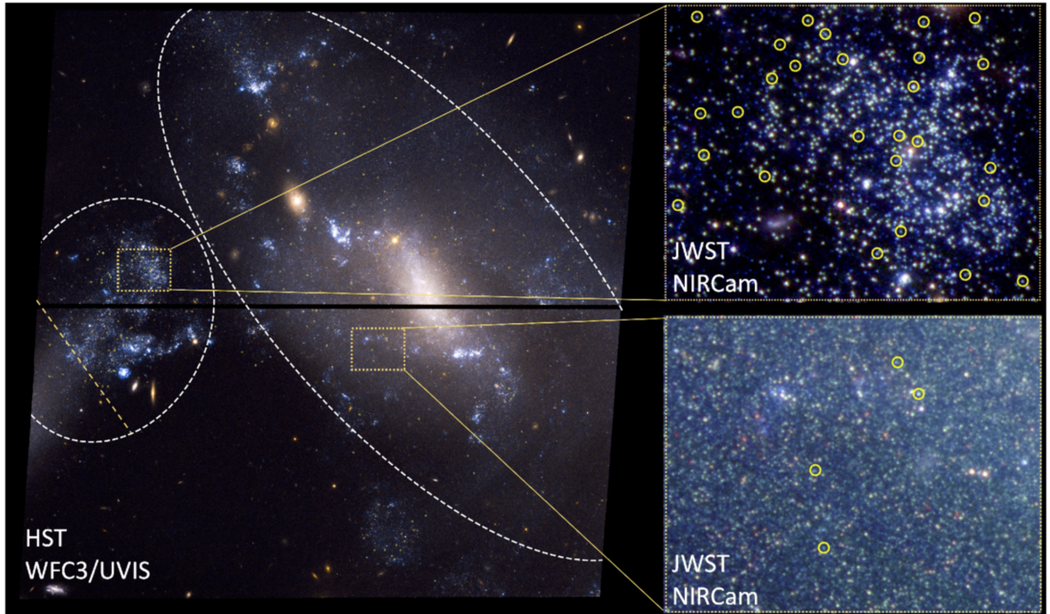
Figure 1. from Adam G. Riess et al 2025 Astrophys. J. Lett. 992 doi:10.3847/2041-8213/ae0ad6 https://dx.doi.org/10.3847/2041-8213/ae0ad6 © 2025. The Author(s). Published by the American Astronomical Society.
