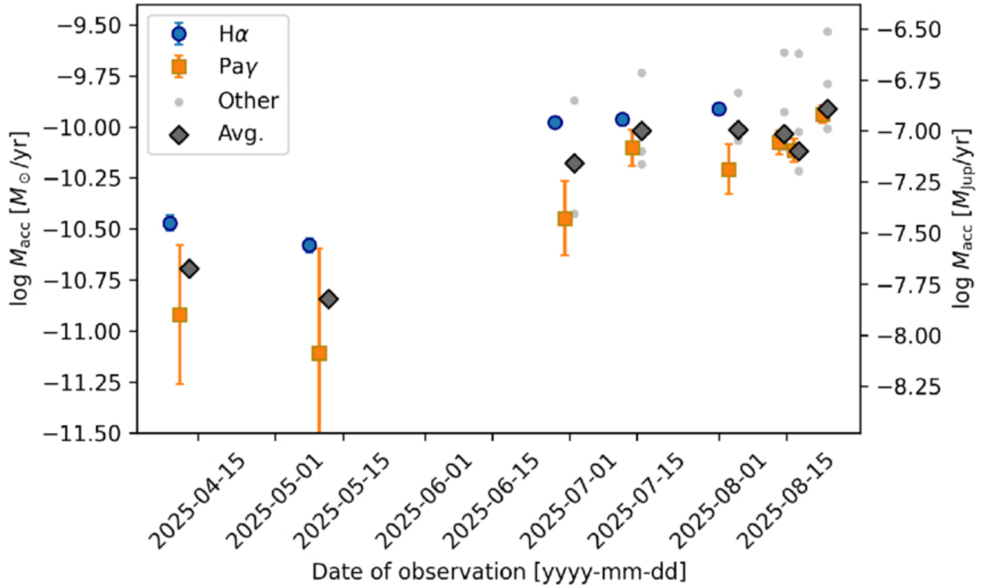
Figure 3. from Victor Almindros-Abad et al 2025 Astrophys. J. Lett. 992 doi:10.3847/2041-8213/ae09a8 https://dx.doi.org/10.3847/2041-8213/ae09a8 © 2025. The Author(s). Published by the American Astronomical Society.
