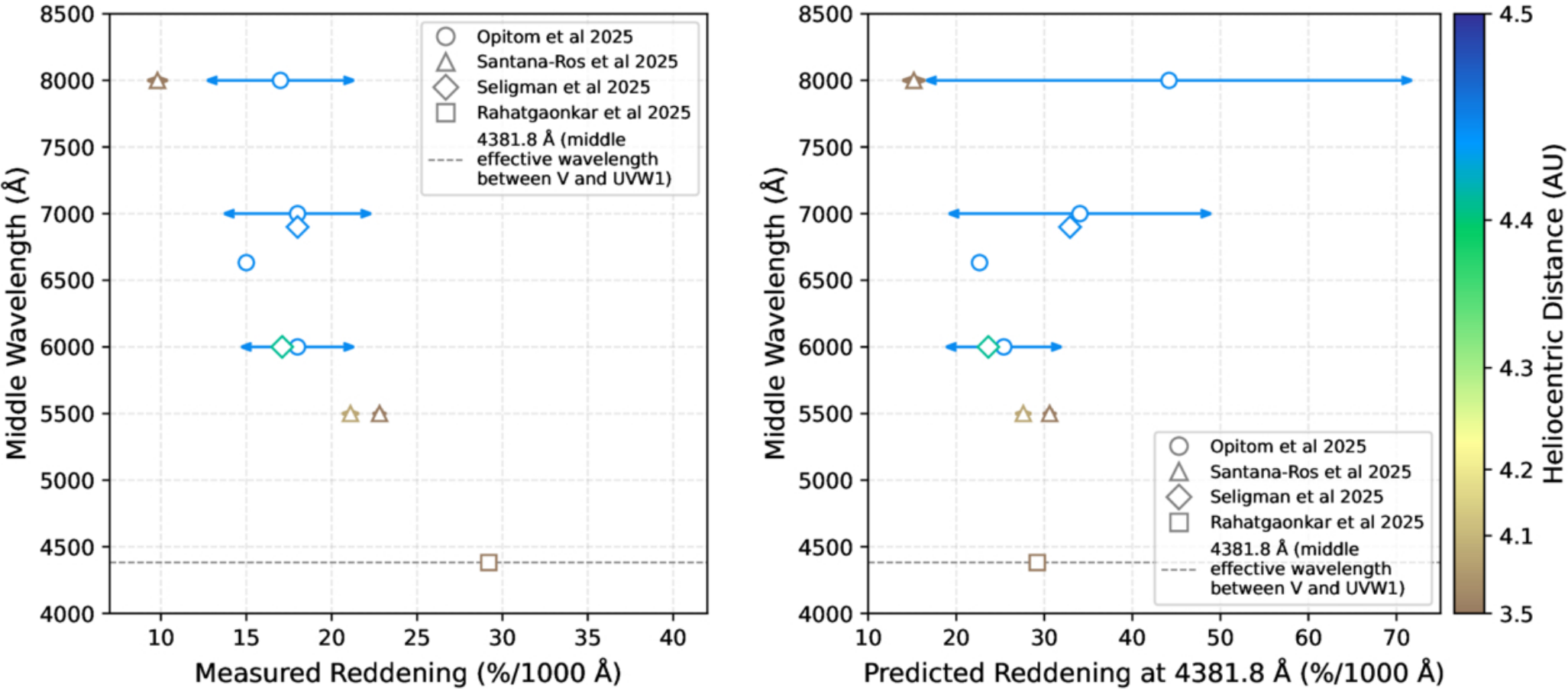
Figure 4. from Zexi Xing et al 2025 Astrophys. J. Lett. 991 doi:10.3847/2041-8213/ae08ab https://dx.doi.org/10.3847/2041-8213/ae08ab © 2025. The Author(s). Published by the American Astronomical Society.
