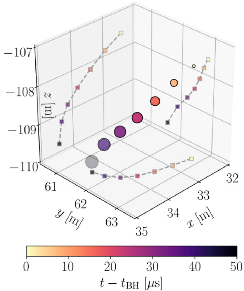
Figure 5. from Goni Halevi et al 2025 Astrophys. J. Lett. 991 doi:10.3847/2041-8213/ae08a6 https://dx.doi.org/10.3847/2041-8213/ae08a6 © 2025. The Author(s). Published by the American Astronomical Society.
