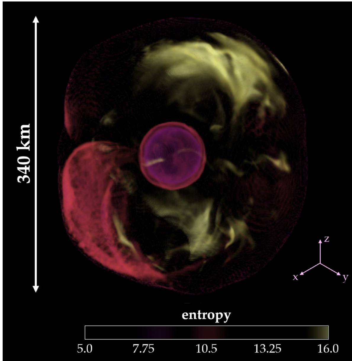
Figure 4. from Goni Halevi et al 2025 Astrophys. J. Lett. 991 doi:10.3847/2041-8213/ae08a6 https://dx.doi.org/10.3847/2041-8213/ae08a6 © 2025. The Author(s). Published by the American Astronomical Society.
