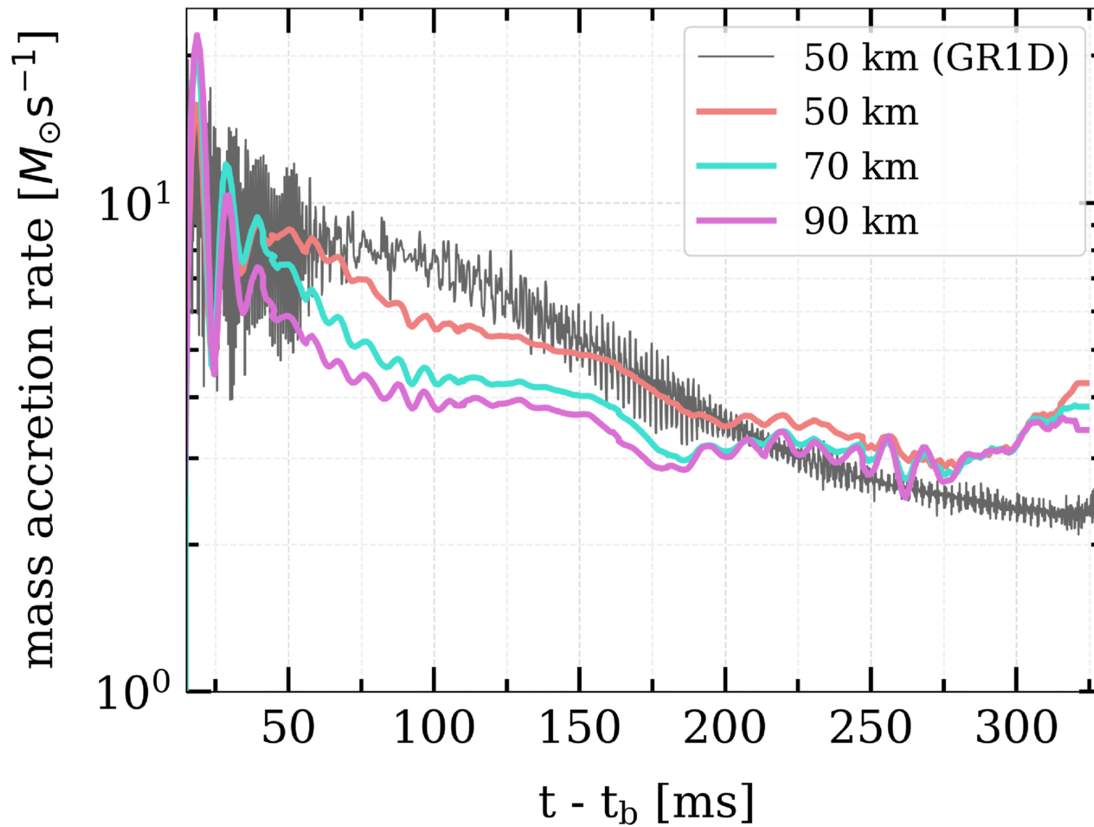
Figure 3. from Goni Halevi et al 2025 Astrophys. J. Lett. 991 doi:10.3847/2041-8213/ae08a6 https://dx.doi.org/10.3847/2041-8213/ae08a6 © 2025. The Author(s). Published by the American Astronomical Society.
