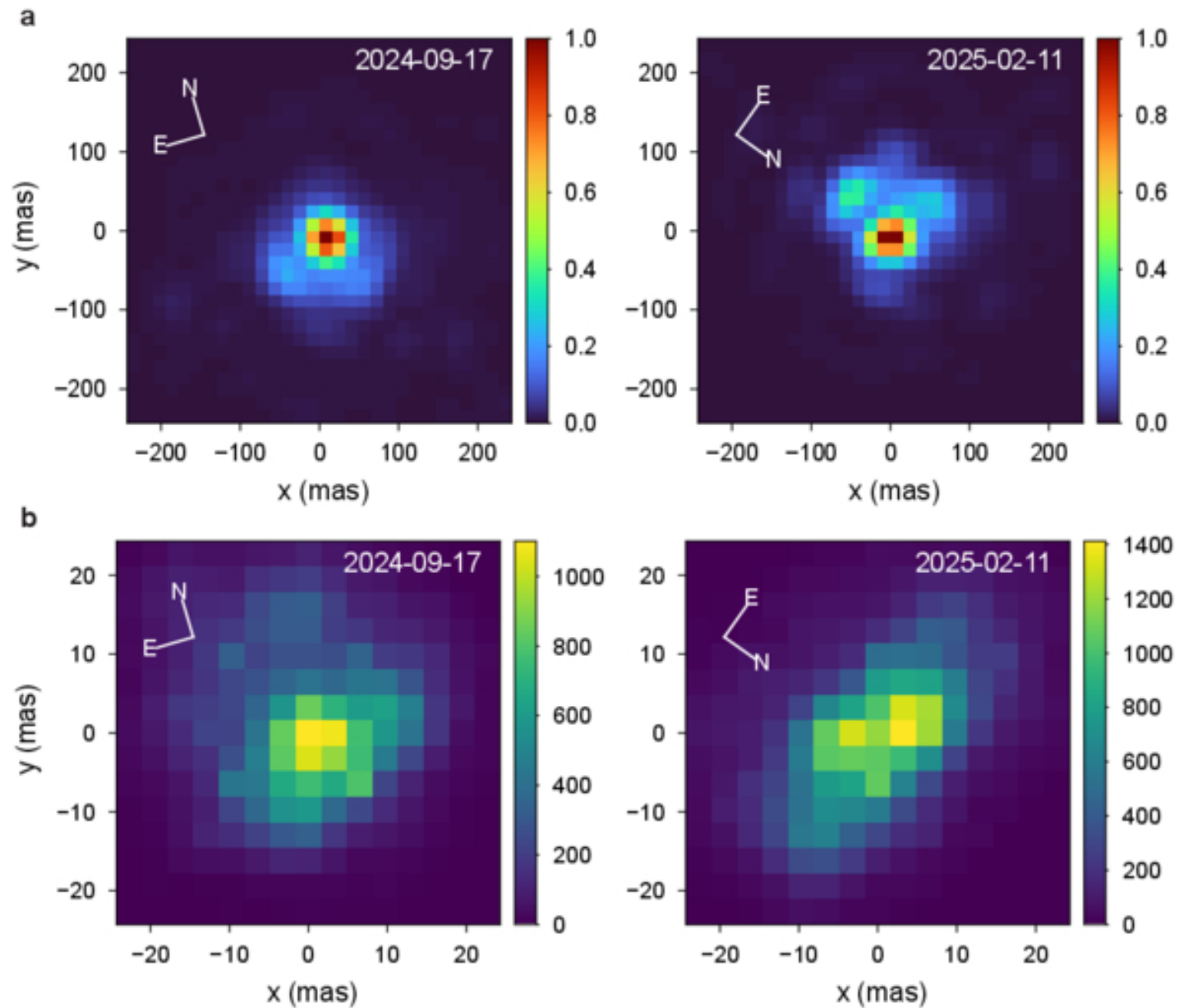
Figure A1. from Yoo Jung Kim et al 2025 Astrophys. J. Lett. 993 doi:10.3847/2041-8213/ae0739 https://dx.doi.org/10.3847/2041-8213/ae0739 © 2025. The Author(s). Published by the American Astronomical Society.
