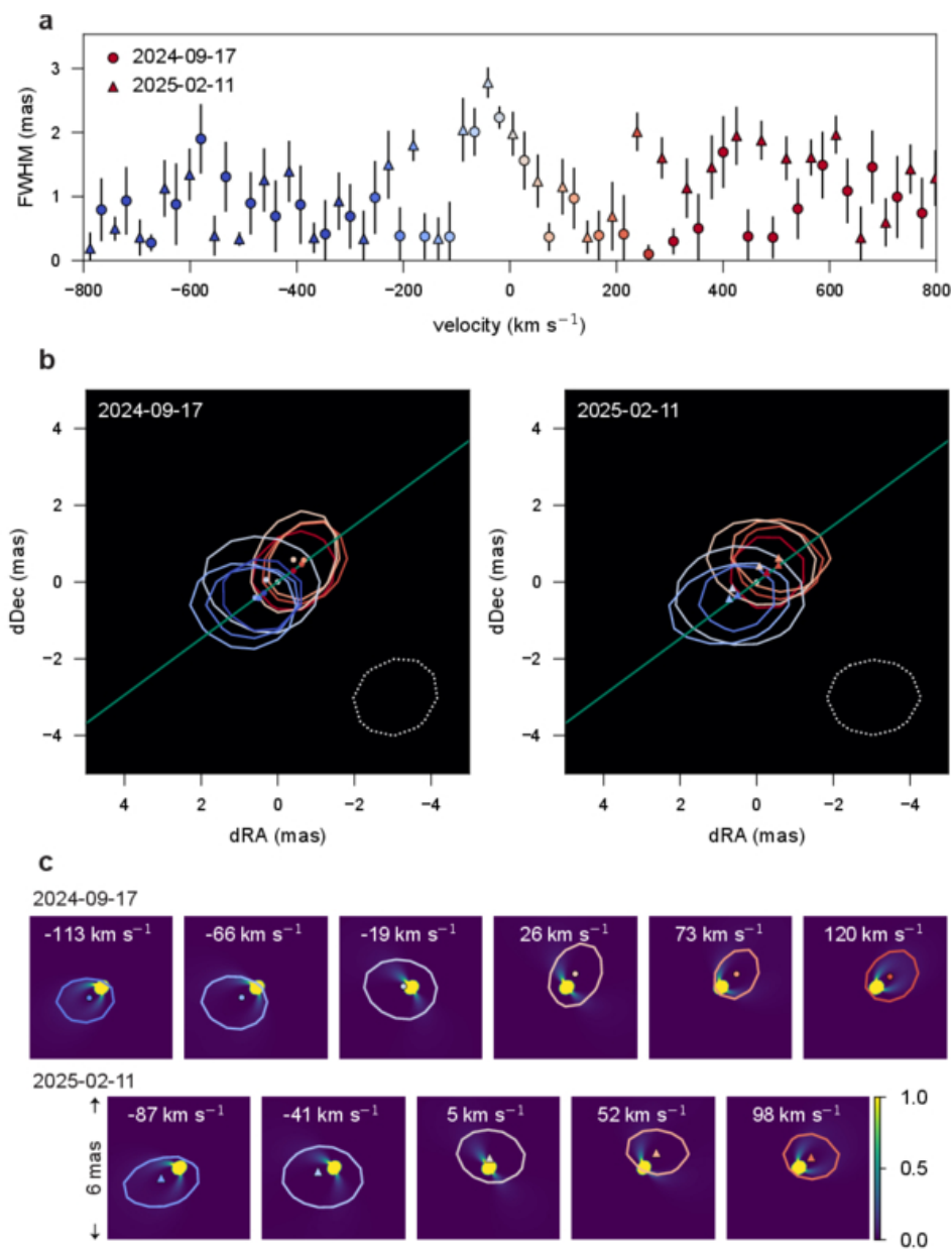
Figure 5. from Yoo Jung Kim et al 2025 Astrophys. J. Lett. 993 doi:10.3847/2041-8213/ae0739 https://dx.doi.org/10.3847/2041-8213/ae0739 © 2025. The Author(s). Published by the American Astronomical Society.
