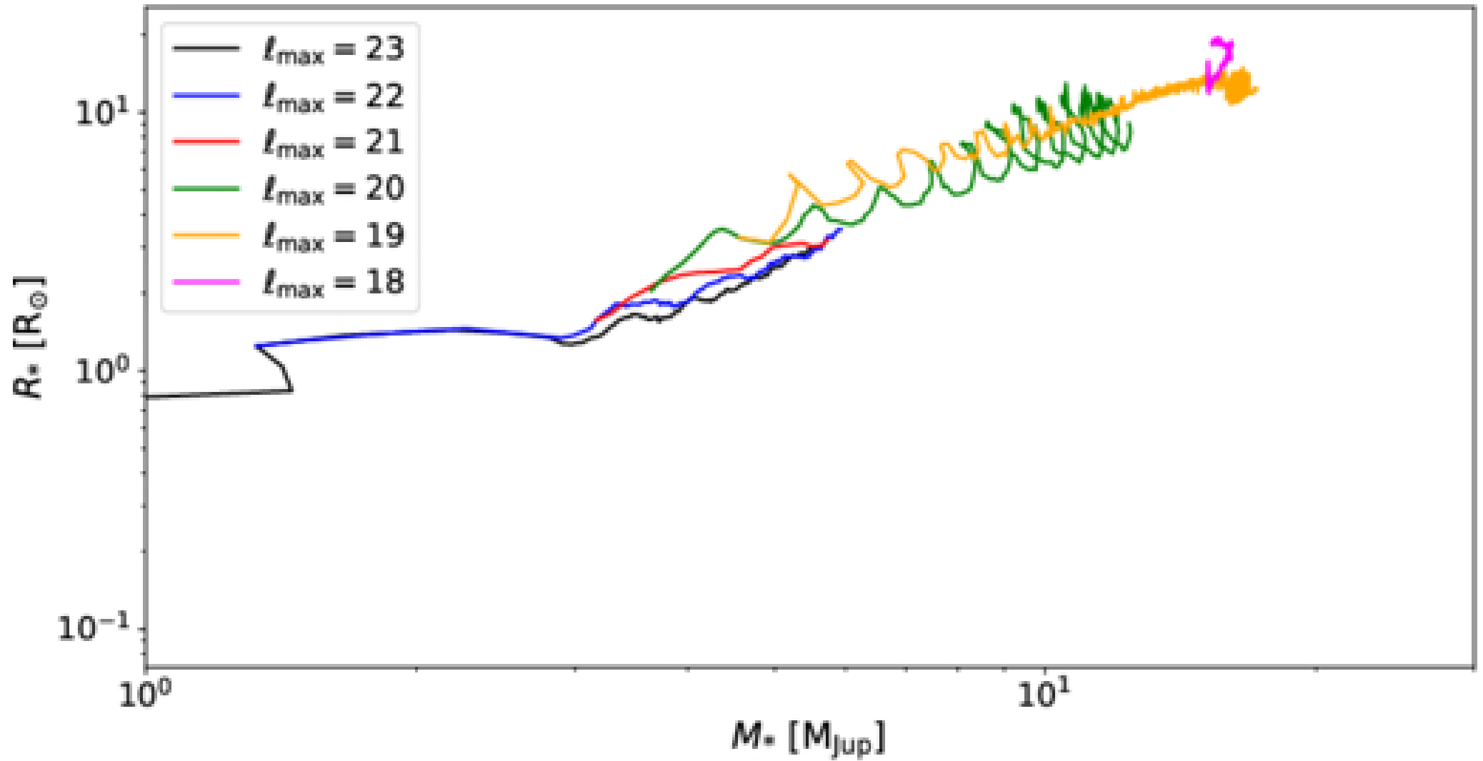
Figure 6. from Adnan Ali Ahmad et al 2025 Astrophys. J. Lett. 991 doi:10.3847/2041-8213/ae0640 https://dx.doi.org/10.3847/2041-8213/ae0640 © 2025. The Author(s). Published by the American Astronomical Society.
