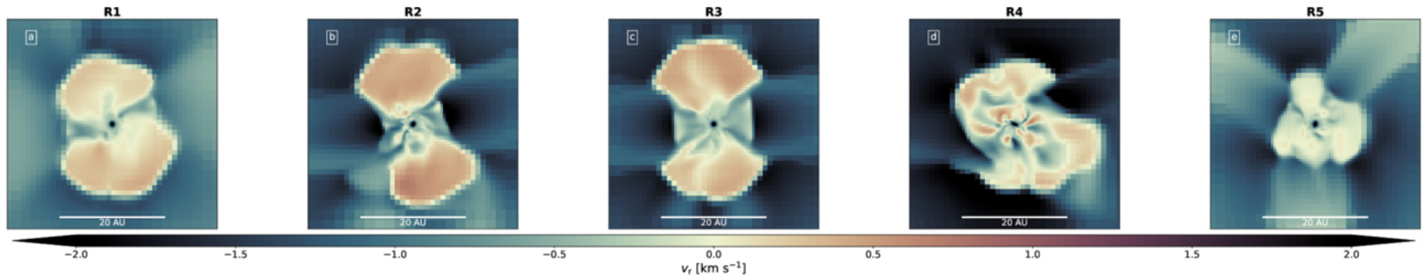
Figure 5. from Adnan Ali Ahmad et al 2025 Astrophys. J. Lett. 991 doi:10.3847/2041-8213/ae0640 https://dx.doi.org/10.3847/2041-8213/ae0640 © 2025. The Author(s). Published by the American Astronomical Society.
