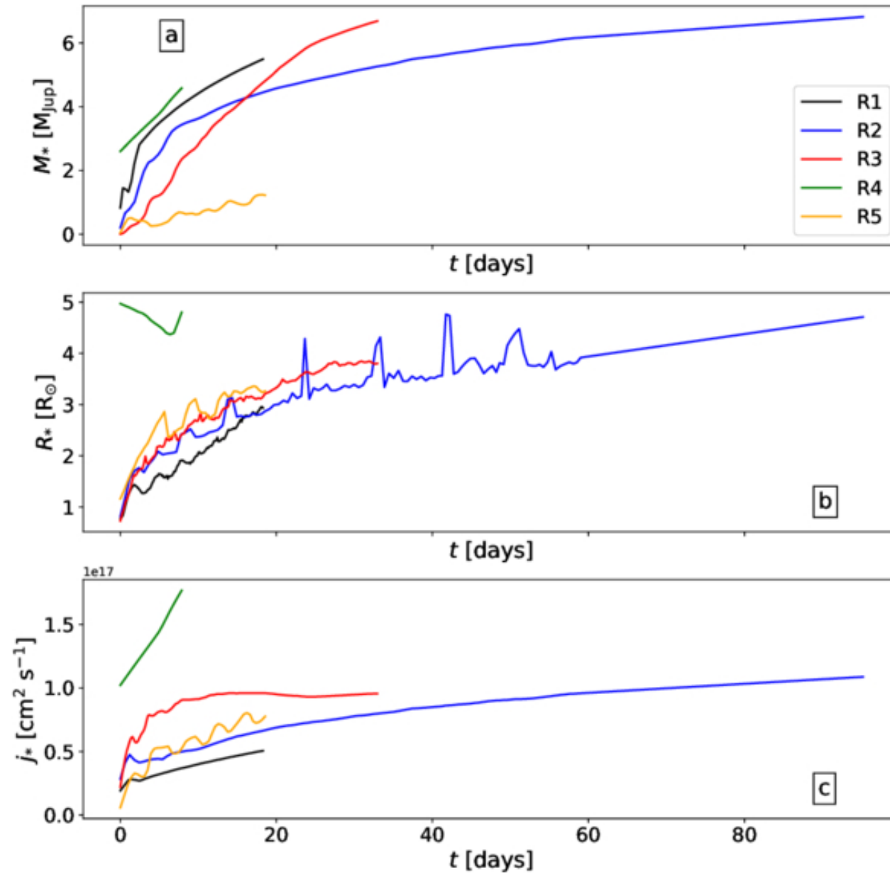
Figure 3. from Adnan Ali Ahmad et al 2025 Astrophys. J. Lett. 991 doi:10.3847/2041-8213/ae0640 https://dx.doi.org/10.3847/2041-8213/ae0640 © 2025. The Author(s). Published by the American Astronomical Society.
