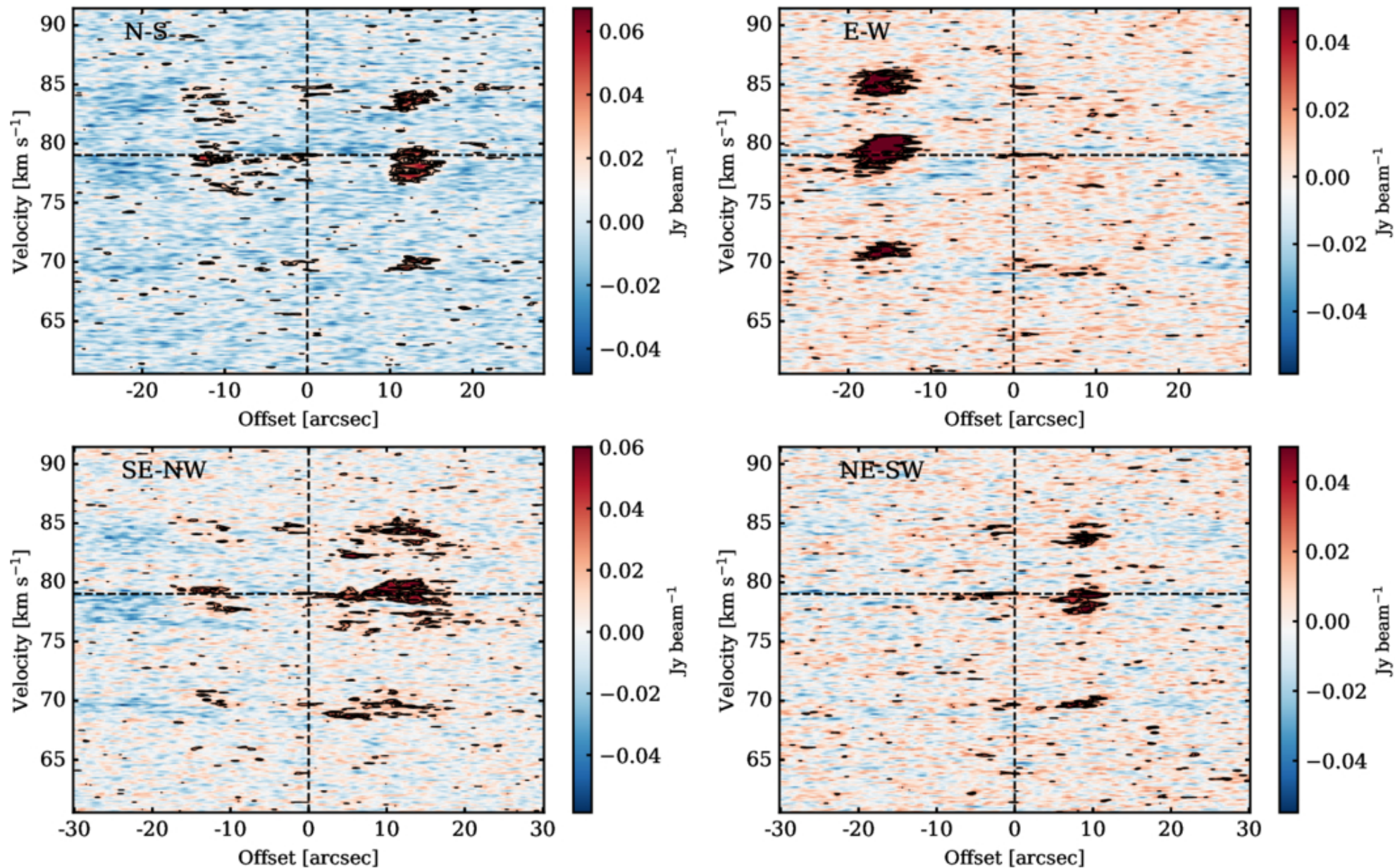
Figure D2. from Shuting Lin et al 2025 Astrophys. J. Lett. 992 doi:10.3847/2041-8213/ae0579 https://dx.doi.org/10.3847/2041-8213/ae0579 © 2025. The Author(s). Published by the American Astronomical Society.
