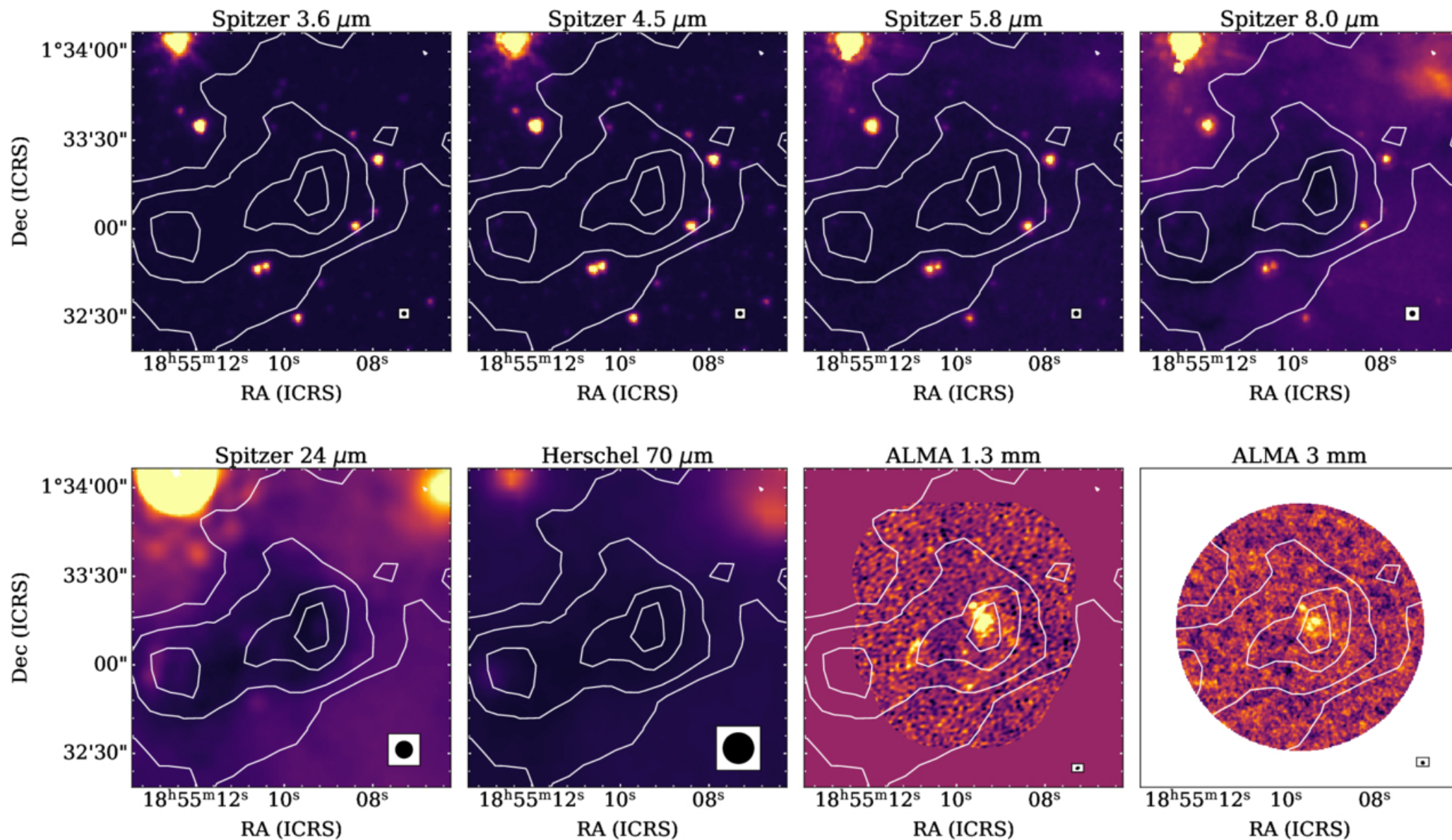
Figure B1. from Shuting Lin et al 2025 Astrophys. J. Lett. 992 doi:10.3847/2041-8213/ae0579 https://dx.doi.org/10.3847/2041-8213/ae0579 © 2025. The Author(s). Published by the American Astronomical Society.
