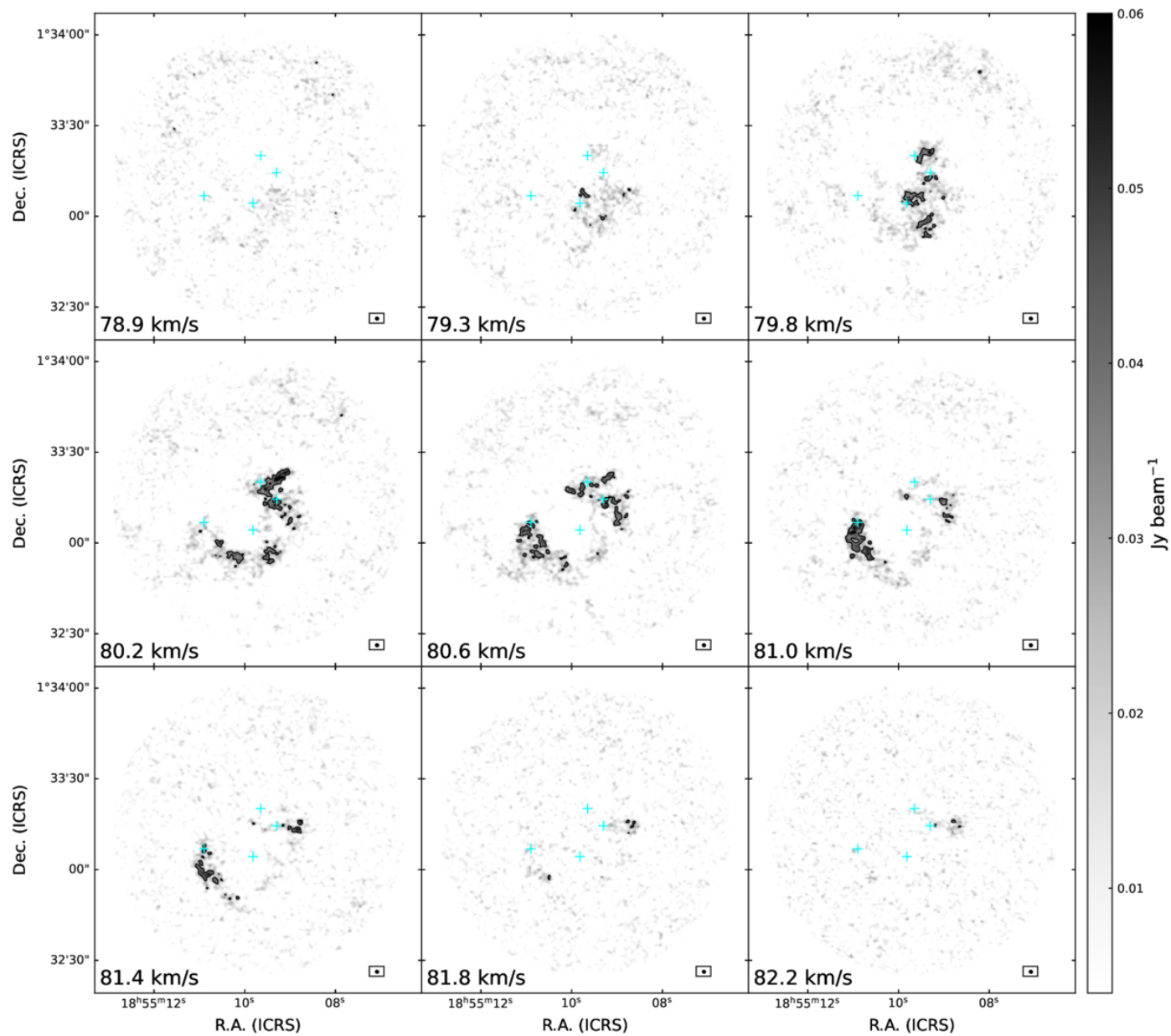
Figure A2. from Shuting Lin et al 2025 Astrophys. J. Lett. 992 doi:10.3847/2041-8213/ae0579 https://dx.doi.org/10.3847/2041-8213/ae0579 © 2025. The Author(s). Published by the American Astronomical Society.
