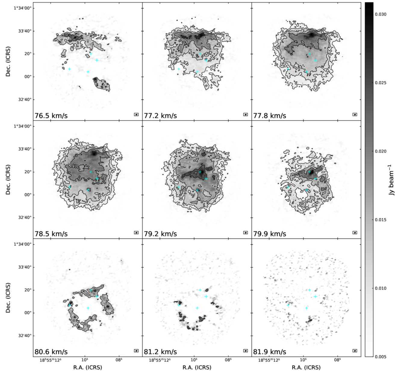
Figure A1. from Shuting Lin et al 2025 Astrophys. J. Lett. 992 doi:10.3847/2041-8213/ae0579 https://dx.doi.org/10.3847/2041-8213/ae0579 © 2025. The Author(s). Published by the American Astronomical Society.
