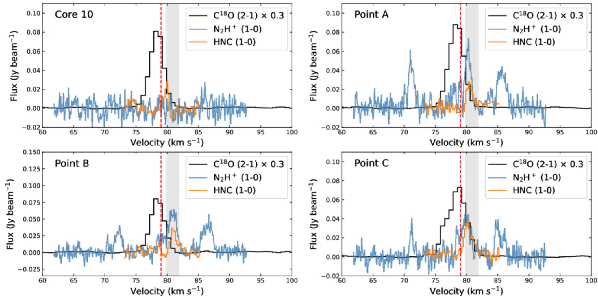
Figure 2. from Shuting Lin et al 2025 Astrophys. J. Lett. 992 doi:10.3847/2041-8213/ae0579 https://dx.doi.org/10.3847/2041-8213/ae0579 © 2025. The Author(s). Published by the American Astronomical Society.
