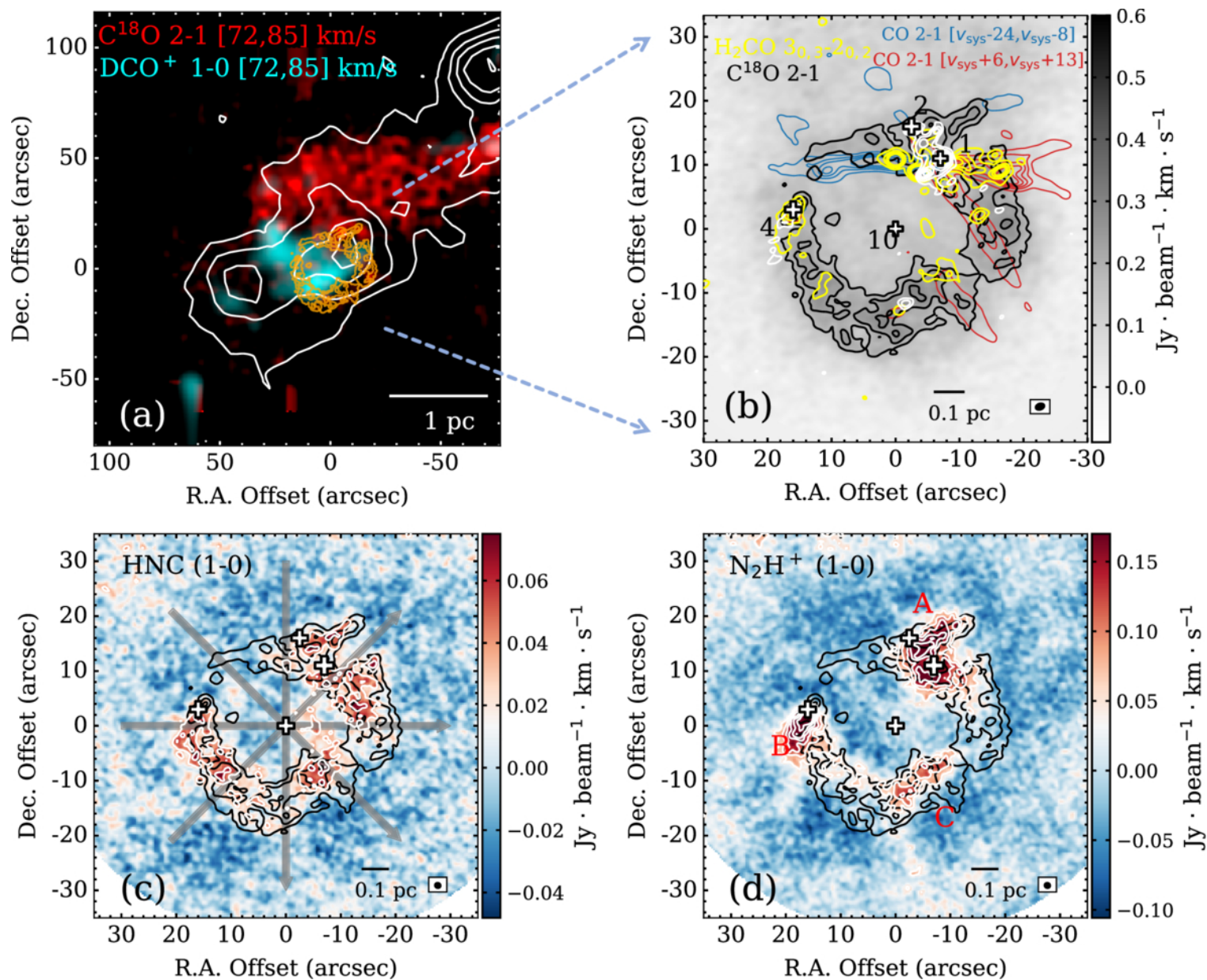
Figure 1. from Shuting Lin et al 2025 Astrophys. J. Lett. 992 doi:10.3847/2041-8213/ae0579 https://dx.doi.org/10.3847/2041-8213/ae0579 © 2025. The Author(s). Published by the American Astronomical Society.
