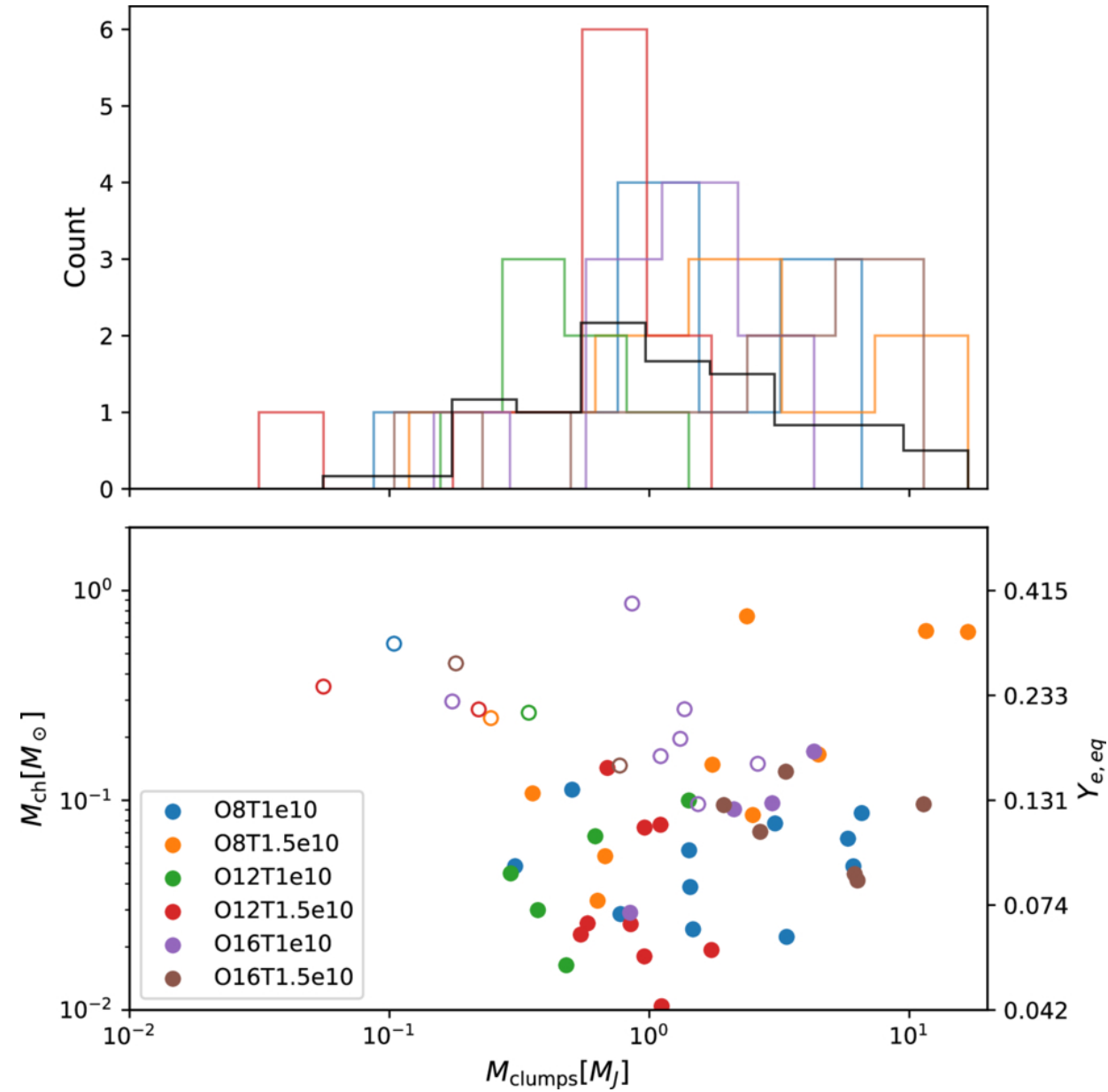
Figure 10. from Yi-Xian Chen and Brian D. Metzger 2025 Astrophys. J. Lett. 991 doi:10.3847/2041-8213/ae045d https://dx.doi.org/10.3847/2041-8213/ae045d © 2025. The Author(s). Published by the American Astronomical Society.
