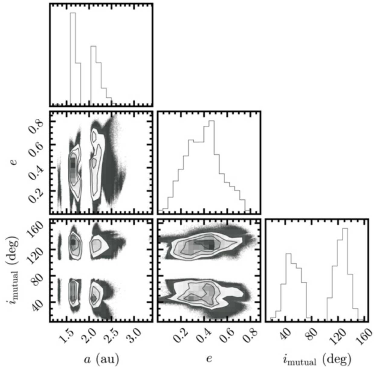
Figure 9. from Charles Beichman et al 2025 Astrophys. J. Lett. 989 doi:10.3847/2041-8213/adf53f https://dx.doi.org/10.3847/2041-8213/adf53f © 2025. The Author(s). Published by the American Astronomical Society.
