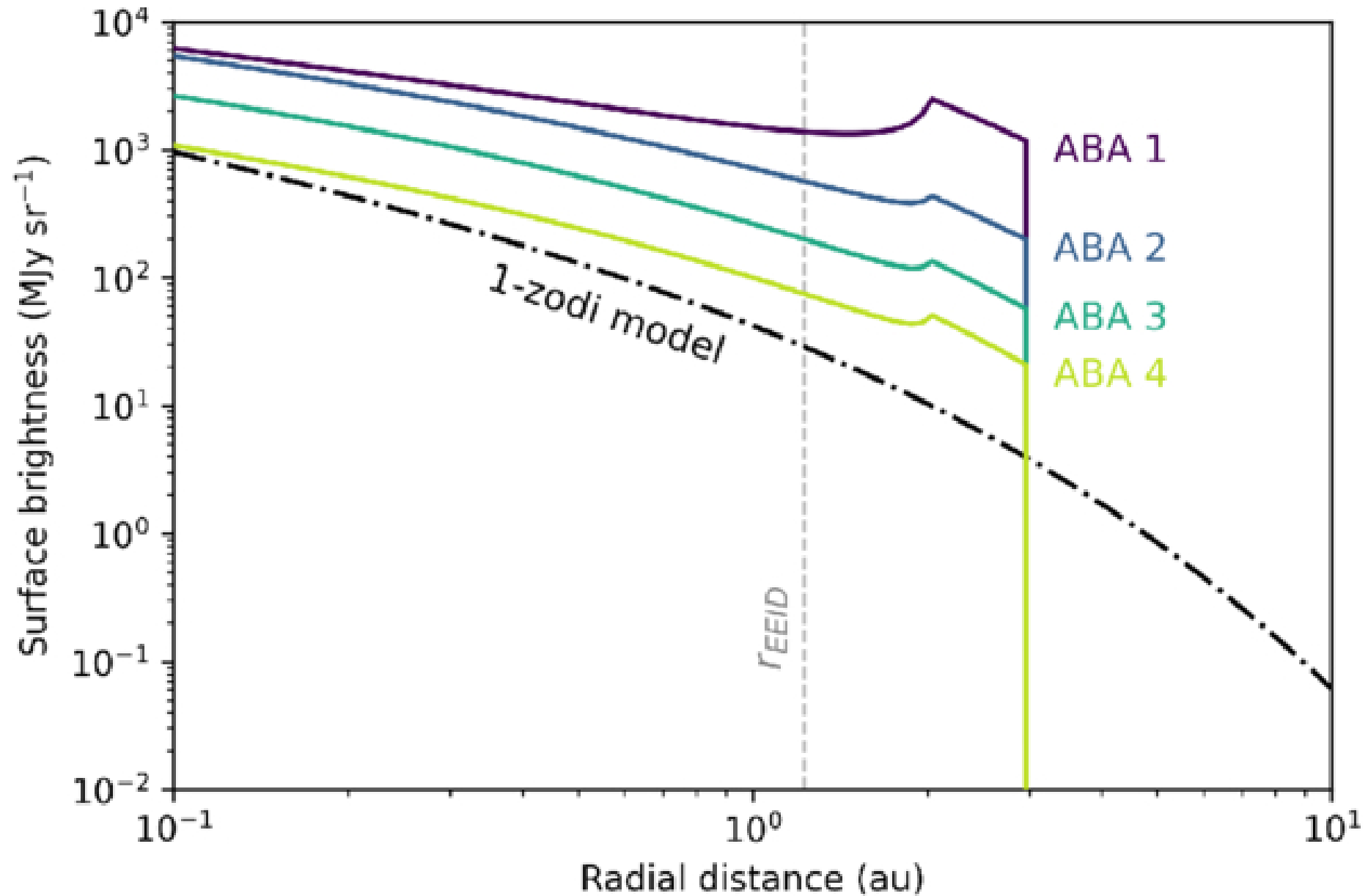
Figure 7. from Charles Beichman et al 2025 Astrophys. J. Lett. 989 doi:10.3847/2041-8213/adf53f https://dx.doi.org/10.3847/2041-8213/adf53f © 2025. The Author(s). Published by the American Astronomical Society.
