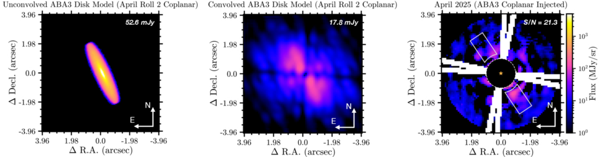
Figure 6. from Charles Beichman et al 2025 Astrophys. J. Lett. 989 doi:10.3847/2041-8213/adf53f https://dx.doi.org/10.3847/2041-8213/adf53f © 2025. The Author(s). Published by the American Astronomical Society.
