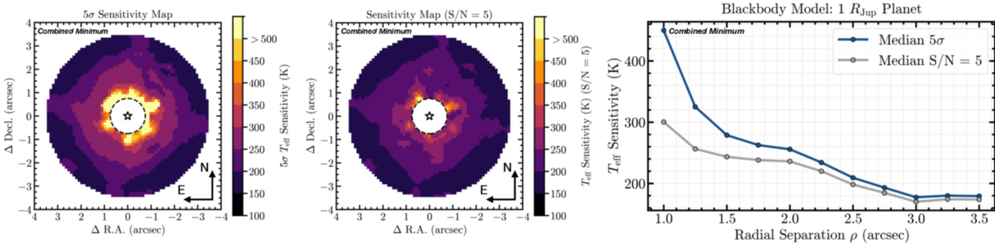
Figure 5. from Charles Beichman et al 2025 Astrophys. J. Lett. 989 doi:10.3847/2041-8213/adf53f https://dx.doi.org/10.3847/2041-8213/adf53f © 2025. The Author(s). Published by the American Astronomical Society.
