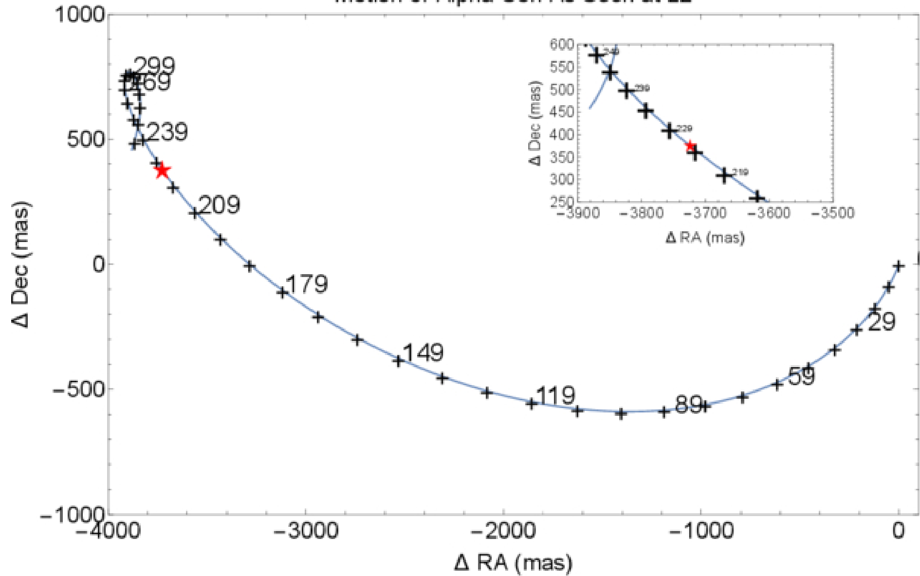
Figure A1. from Charles Beichman et al 2025 Astrophys. J. Lett. 989 doi:10.3847/2041-8213/adf53f https://dx.doi.org/10.3847/2041-8213/adf53f © 2025. The Author(s). Published by the American Astronomical Society.
