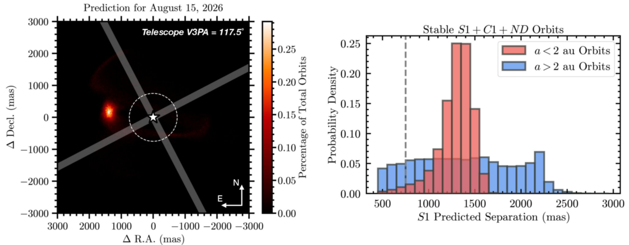
Figure 19. from Charles Beichman et al 2025 Astrophys. J. Lett. 989 doi:10.3847/2041-8213/adf53f https://dx.doi.org/10.3847/2041-8213/adf53f © 2025. The Author(s). Published by the American Astronomical Society.
