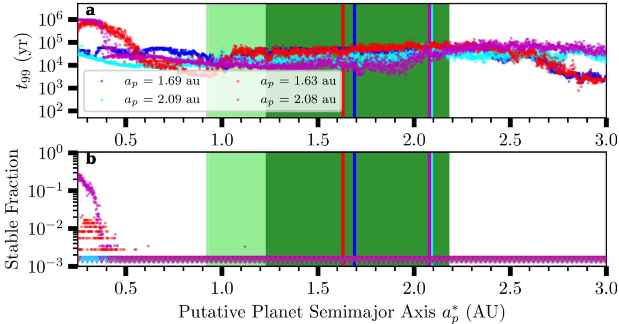
Figure 18. from Charles Beichman et al 2025 Astrophys. J. Lett. 989 doi:10.3847/2041-8213/adf53f https://dx.doi.org/10.3847/2041-8213/adf53f © 2025. The Author(s). Published by the American Astronomical Society.
