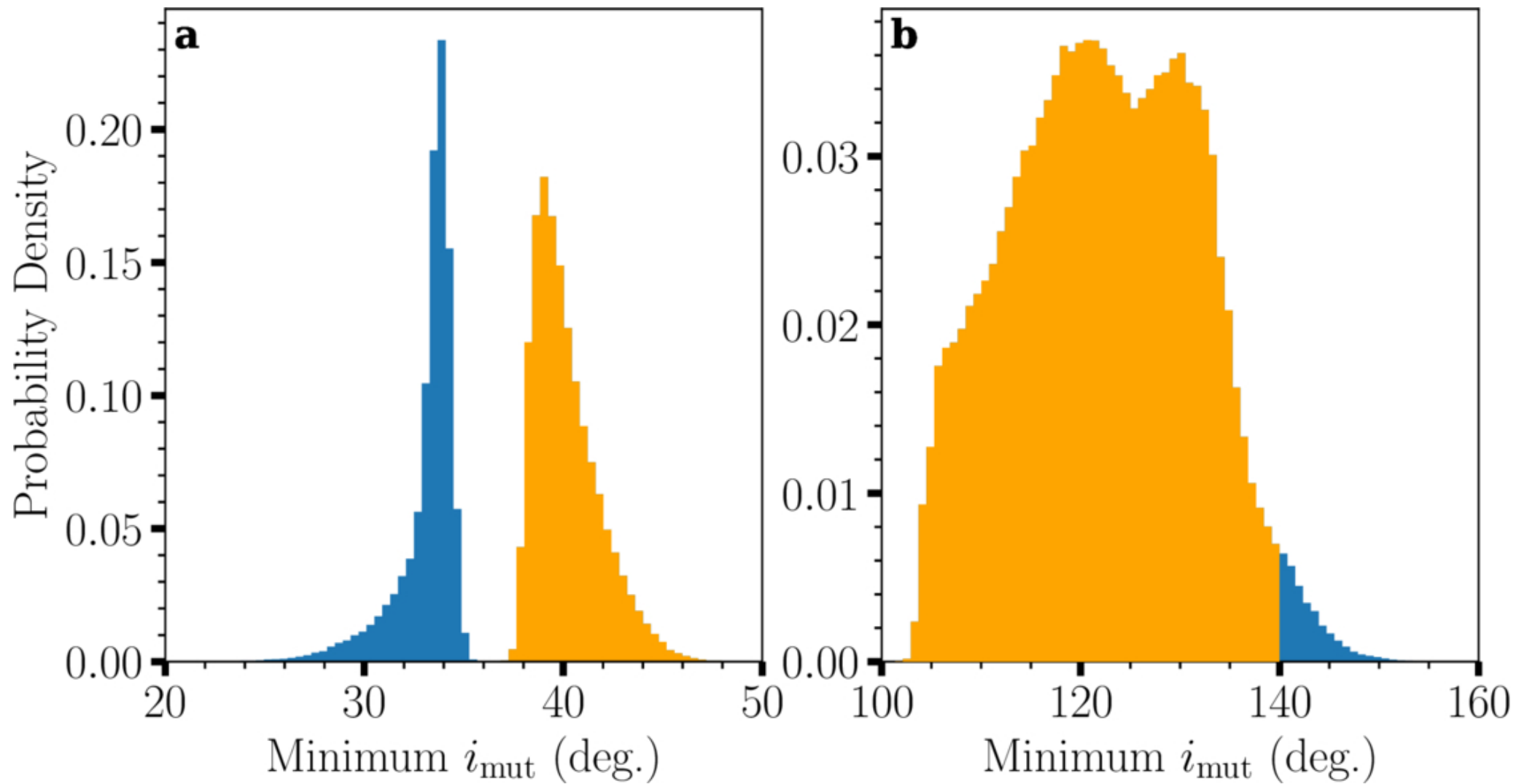
Figure 17. from Charles Beichman et al 2025 Astrophys. J. Lett. 989 doi:10.3847/2041-8213/adf53f https://dx.doi.org/10.3847/2041-8213/adf53f © 2025. The Author(s). Published by the American Astronomical Society.
