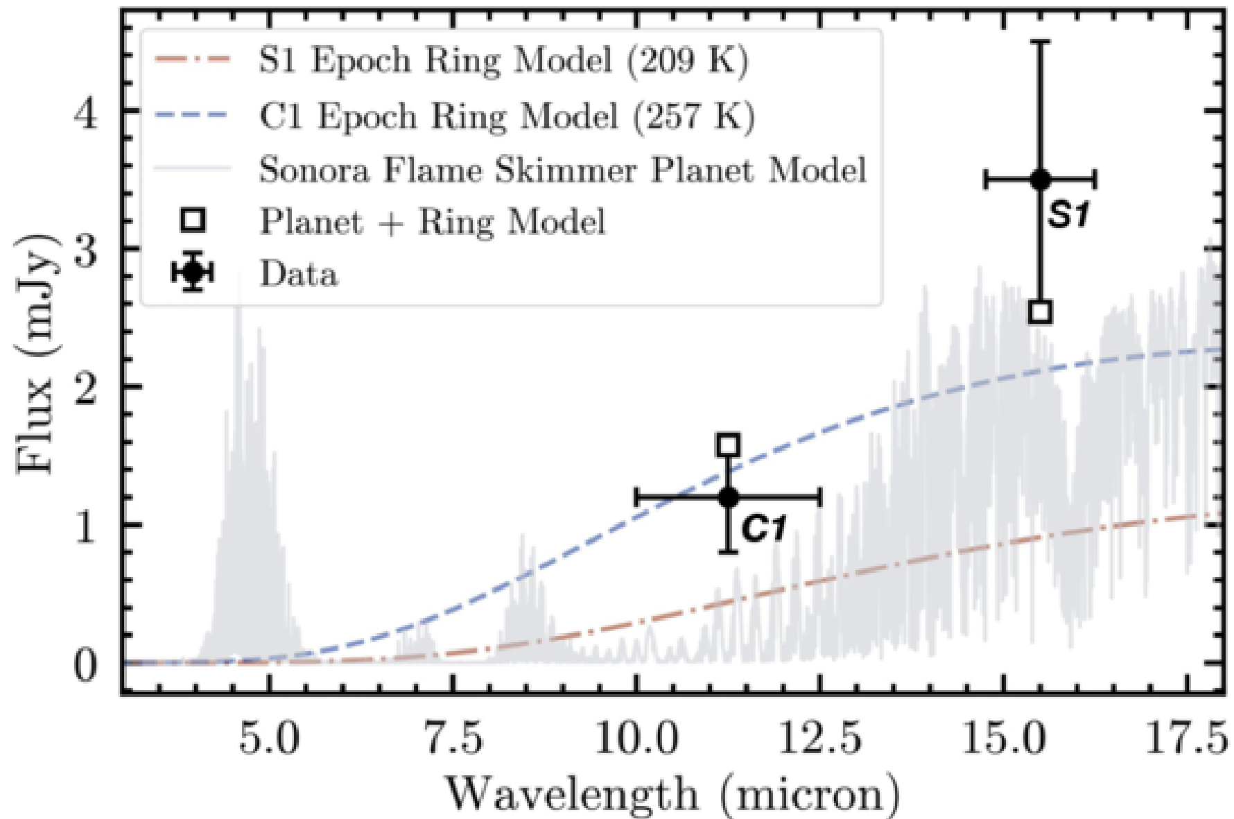
Figure 15. from Charles Beichman et al 2025 Astrophys. J. Lett. 989 doi:10.3847/2041-8213/adf53f https://dx.doi.org/10.3847/2041-8213/adf53f © 2025. The Author(s). Published by the American Astronomical Society.
